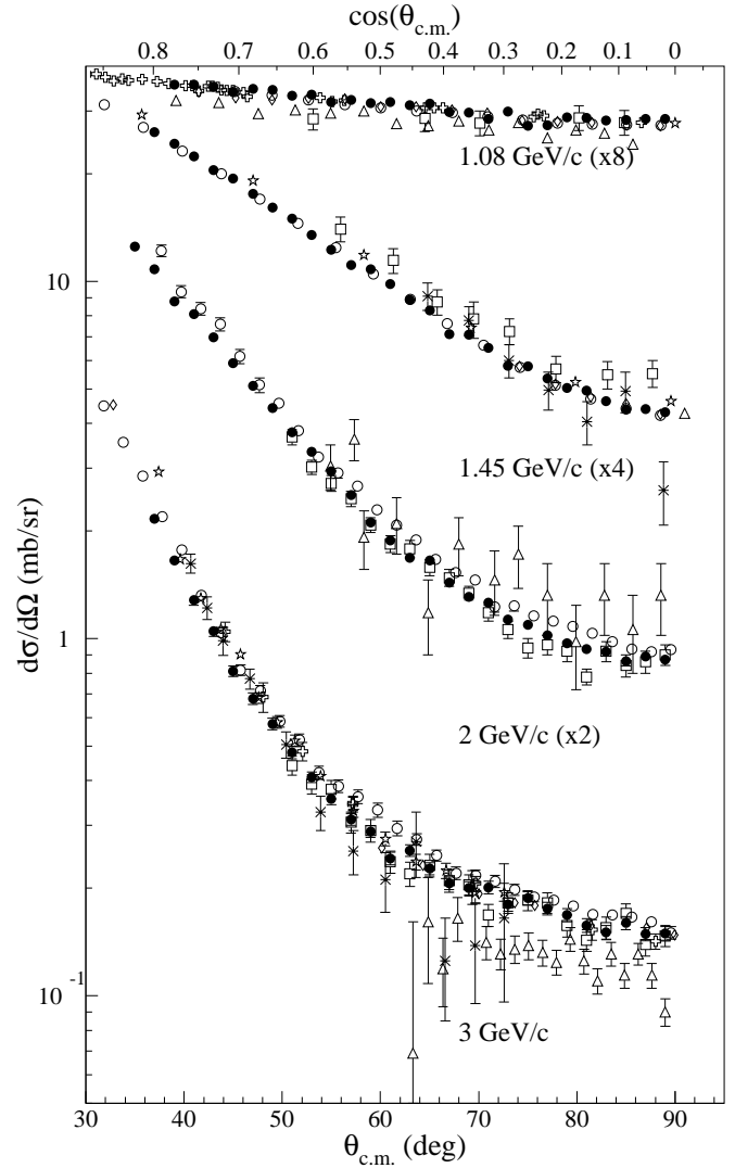
Fig. 26. Angular distributions at four beam momenta. Data of this work (●) are compared to published data, where the symbols ○, □, △, ◇, ◻, ☆, and * correspond to data from [30, 48, 50, 51, 52, 53] at 1.08 GeV/c, [30, 48, 49, 51, 54, 55, 56] at 1.45 GeV/c, [46, 47, 57] at 2 GeV/c and [45, 46, 47, 58, 59, 60, 61] at 3 GeV/c.
