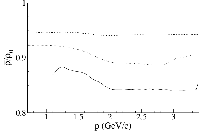
Fig. 17. Average relative hydrogen density as a function of momentum for three samples corresponding to different setups of the COSY beam.
