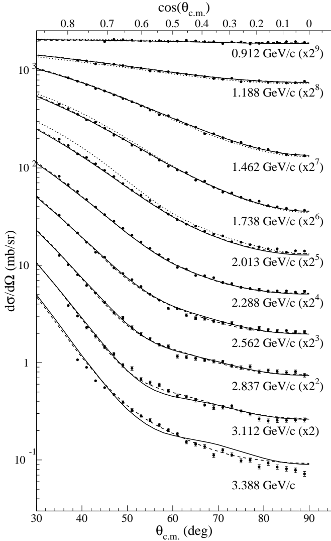
Fig. 25. Angular distributions of d\sigma/d\Omega_{c.m.} (●: data of this work) for ten beam momenta p in in comparison to SAID solutions (cf. Fig. 23).
