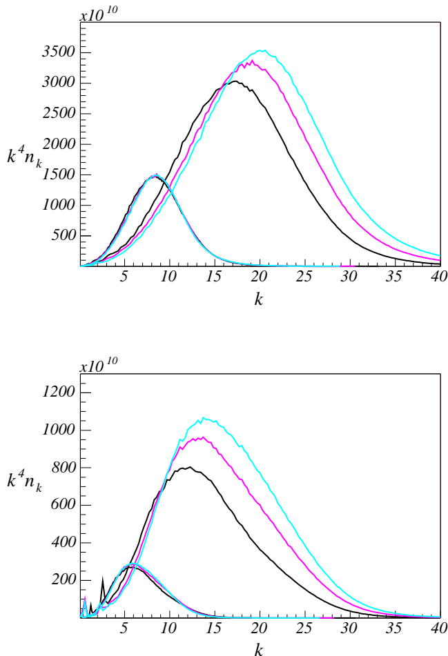
FIG. 5: Spectral energy distributions for \chi (upper panel) and \phi (lower panel) in the model with h = 10g . In each panel we plot the wave energy per decade found in lattice integrations at three moments of time, \eta = 1000, 1500 and 2000 . In the lower-left corner of each panel are the same graphs transformed according to the relation inverse to Eq. (4).
