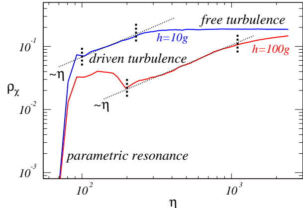
FIG. 6: Different regimes of the evolution of the \chi field for two values of self-coupling, h = 10g and h = 100g . The dashed lines correspond to a linear growth of energy in the \chi field with time, \rho_\chi \propto \eta .
