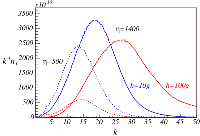
FIG. 7: Spectral energy distributions at two moments of time, \eta = 500 (dotted lines) and \eta = 1400 (solid lines). We compare two models with different self-coupling, h = 10g and h = 100g .
