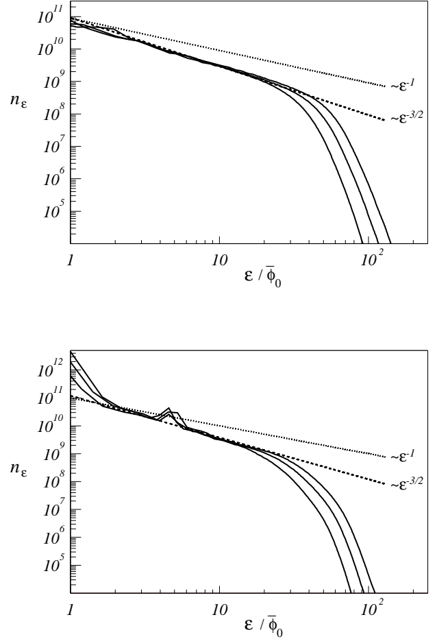
FIG. 4: Particle distributions in the self-similar regime for h = 10g as functions of the corresponding wave kinetic energies rescaled by the current zero-mode amplitude \bar{\phi}_0 . Upper and lower panels correspond to \chi and \phi fields respectively. In both cases from left to right the plots are taken at \eta = 1000, 1500, 2000 .
