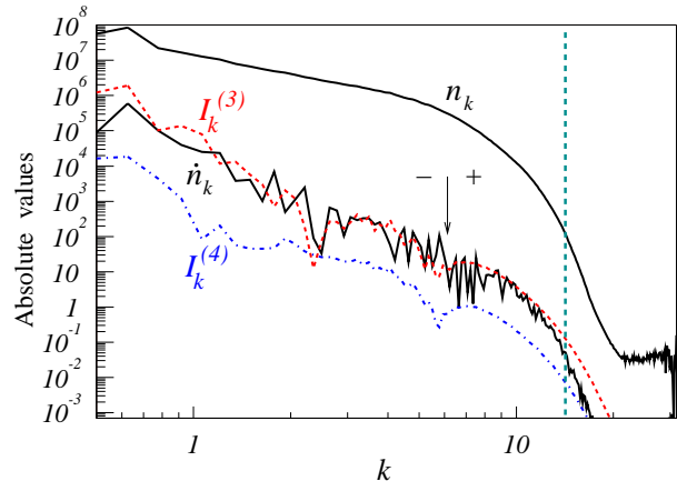
FIG. 8: Absolute values of \dot{n}(k) and of I_k^{(3)} and I_k^{(4)} collision integrals at \eta = 5000 . To the left of the arrow \dot{n}(k) and collision integrals are negative, while to the right they are positive. Occupation numbers, n_k , are also shown for comparison. I_k^{(3)} agrees with \dot{n}(k) to the left of the vertical dashed line.
