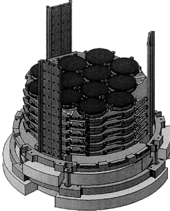
Fig. 5. Drawing of the EDELWEISS-II detector set-up. Up to 120 Ge detectors of mass 320 g (the blue plates) can be accommodated in a compact hexagonal arrangement at 10 mK. The grey plate, made of ultra-pure archeological lead, shields the detectors from the radioactivity of the dilution cryostat (not shown).
