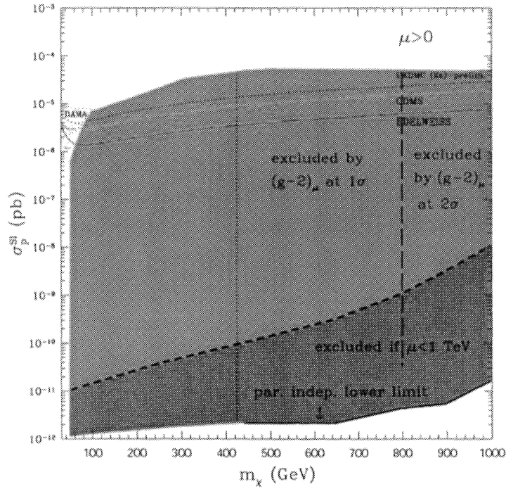
Fig. 2. Experimental sensitivities of the present most sensitive WIMP direct detection experiments (from Ref. [19] ). The EDELWEISS result, without background subtraction, excludes the full 3\text{-}\sigma zone of the DAMA signal (upper left corner) compatible with accelerator constraints, independently of the WIMP halo model parameters. The parameter independent lower limit on the WIMP-p cross-section can be seen to be \sim 10^{-12} pbarn.
