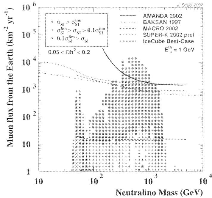
Fig. 4. Sensitivities of the present and future indirect searches using interactions of neutrinos produced in WIMP annihilations in the Earth (from Ref. [26] ) compared with the sensitivity obtained by the EDELWEISS direct search (noted SI (spin-independent), region represented by full grey dots). Improvement in the sensitivity of direct detection experiments by a factor 10 will allow to sample the region marked with + symbols. The target sensitivities of the future ICECUBE experiment is also presented on the figure as the lower dotted curve.
