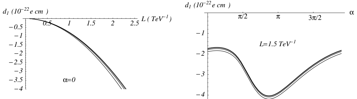
FIG. 2: Left: The fermionic EDM, d_1 , in units of 10^{-22} e \text{ cm} for the zero-mode of the fermion i = 1 as a function of the compactification length L in units of \text{TeV}^{-1} for \alpha = 0 . Right: Same, as a function of \alpha for L = 1.5 \text{ TeV}^{-1} . The curves from the bottom to the top correspond to the number of modes included in (23) varying from |n| = 1 to |n| = 4 ; the fast convergence of the series is evident. Note that the mass of the zero-mode also varies with L . We used e = \sqrt{4\pi\alpha_{QED}} and the same parameters as in Fig. 1.
