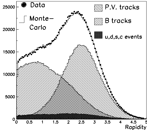
Figure 2: Distributions of rapidity from 1994 data and simulation where the normalisation is to the number of entries. From the simulation, tracks originating at the primary vertex and tracks from the b-hadron decay chain are also plotted.
