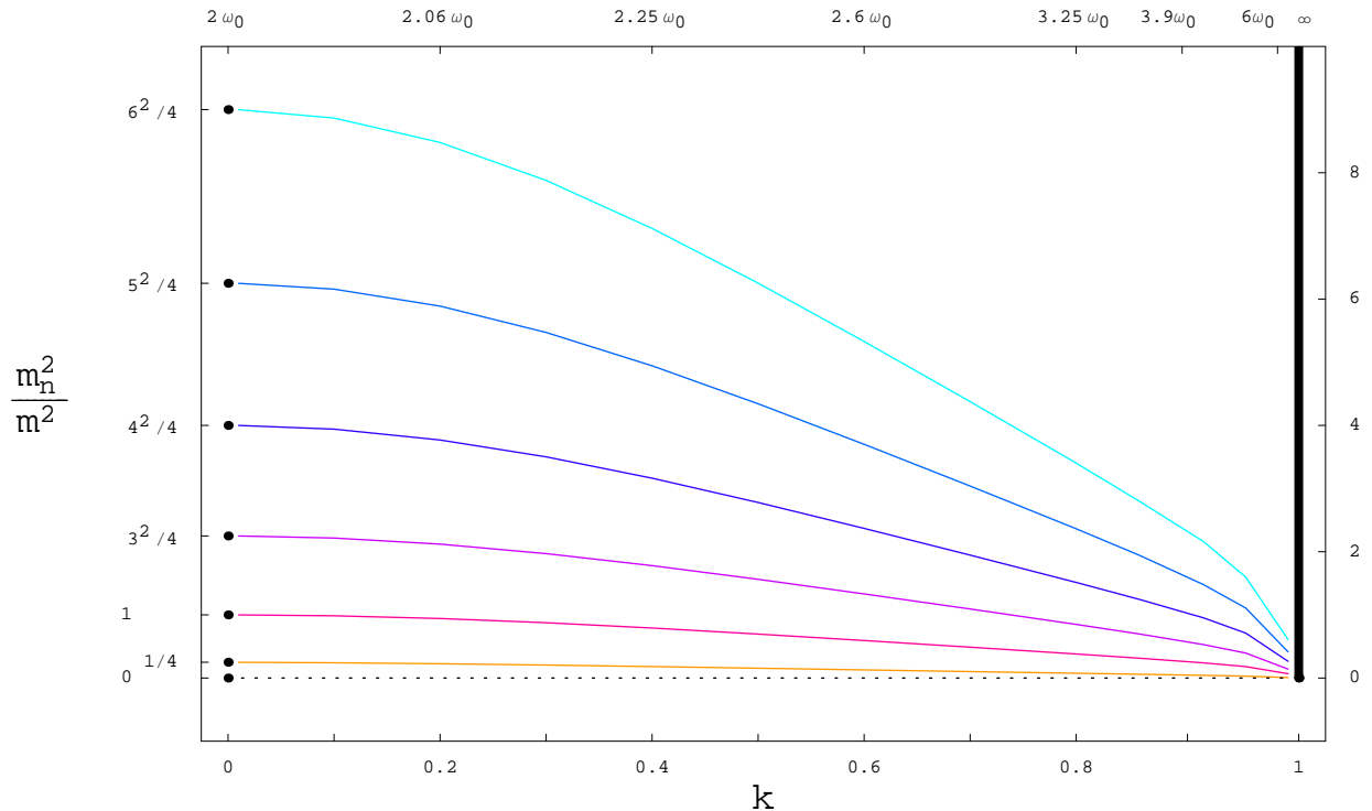
Figure 5: The mass variation of the first 7 modes with respect to the size of the extra dimension (i.e. the value of k ). The spectrum goes from the discrete n^2 type spectrum at k = 0 to the continuum spectrum for the case k = 1 , represented by the thick black vertical line. Here we have taken \delta = 0.1
