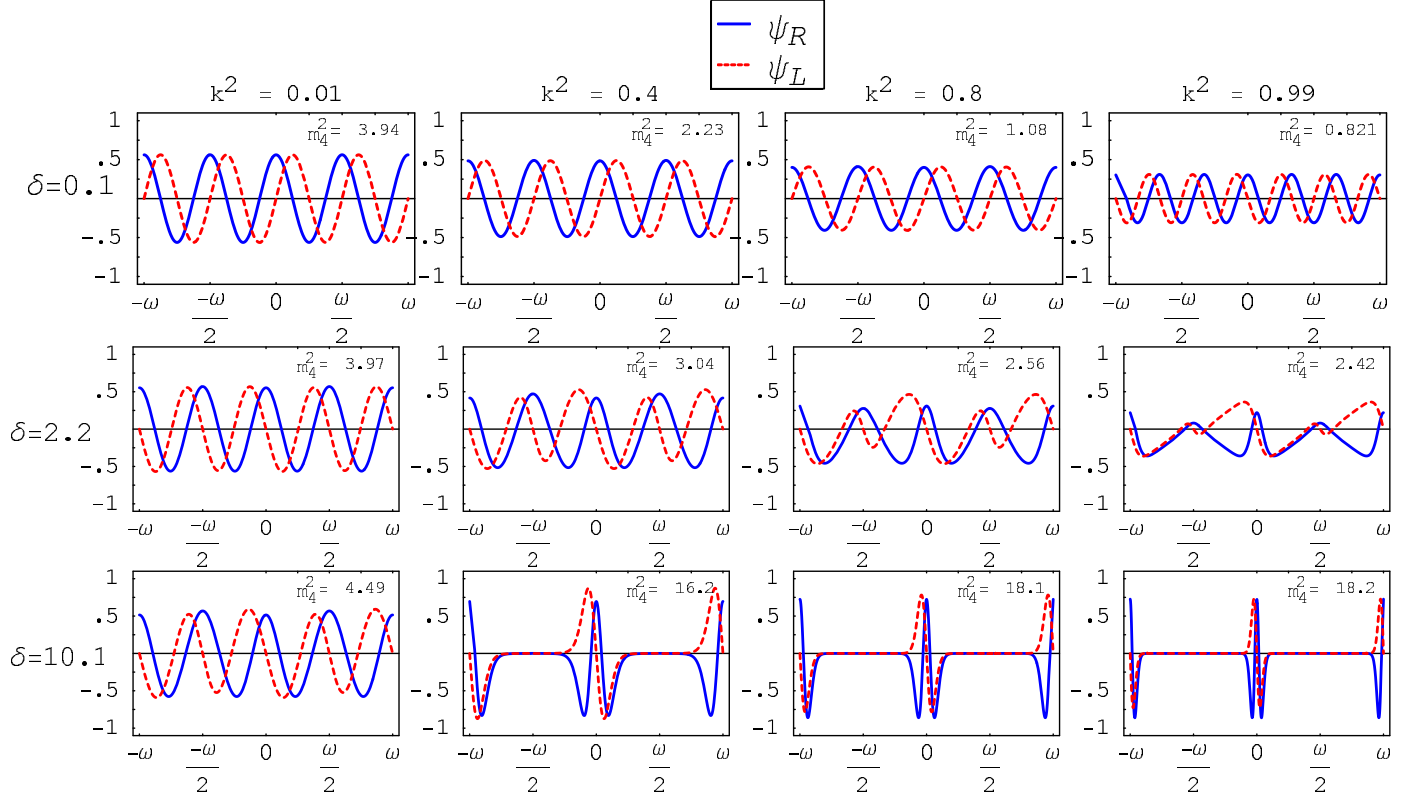
Figure 11: The profile of the normalized mode \psi_4^{\text{R/L}} , of period \omega , for k^2 = 0.01, 0.4, 0.8 and 0.99 (or \omega = 1.01\omega_0, 1.34\omega_0, 1.93\omega_0 and 3.32\omega_0 , with \omega_0 = 2\pi/m ) and with \delta = 0.1, 2.2 and 10.1 . The mass eigenvalues are given in units of m^2 .
