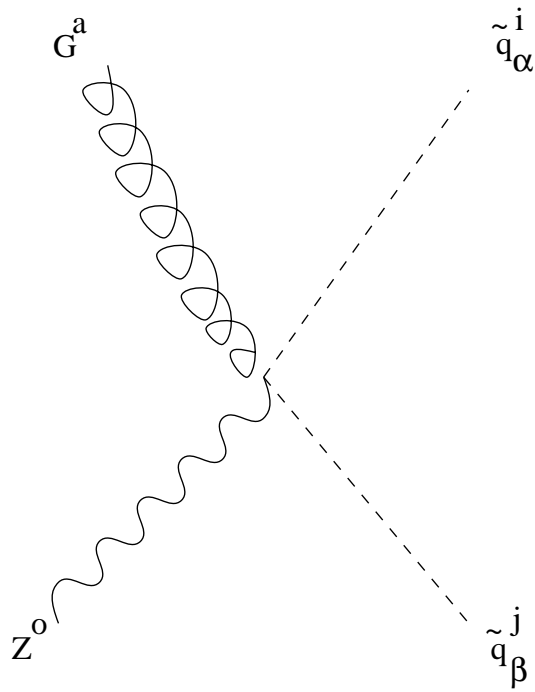
Figure 35: 2g_3 \frac{g_2}{\cos w} T_{ij}^a F^{2I} (T_{3I} \mp \sin^2 w)
