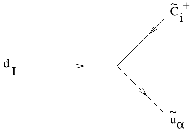
Figure 13: +g_2 V_{JI}^{CKM} (S_{UL}^{CKM})_J V_{i1} C^1 P_L + \frac{g_2}{2m_W \cos} V_{JI}^{CKM} (S_{UL}^{CKM})_J m_I^d U_{i2} C^1 P_R + \frac{g_2}{2m_W \sin} V_{JI}^{CKM} (S_{UR}^{CKM})_J m_J^u V_{i2} C^1 P_L
