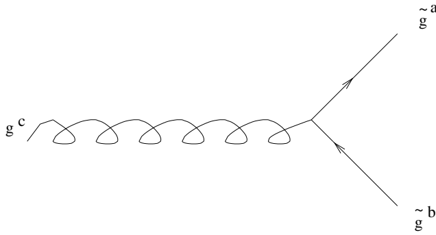
Figure 22: ig_3 f_{abc}
