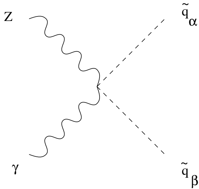
Figure 31: \frac{2geq_e}{\cos \theta_w} F^{2I} (T_{3I} - q \sin^2 \theta_w)
