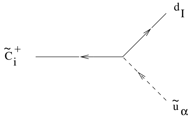
Figure 11: \frac{g}{2m_W \cos} (V^{CKM})_{IJ}^Y (S^{CKM})_{UL}^J V_{i1} \not{P} + \frac{g_2}{2m_W \sin} (V^{CKM})_{IJ}^Y (S^{CKM})_{UR}^J m_J^u V_{i2} \not{P} + \frac{g_2}{2m_W \cos} (V^{CKM})_{IJ}^Y (S^{CKM})_{UL}^J m_I^d U_{i2} \not{P}
