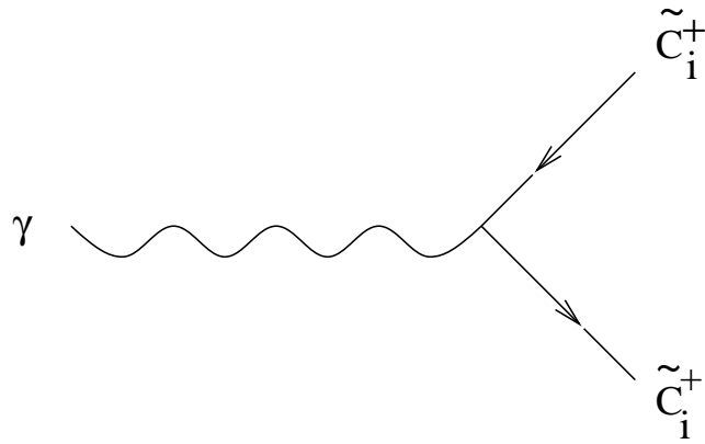
Figure 19: e
