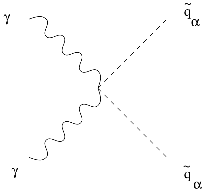
Figure 29: 2e^2 e_q^2 g
