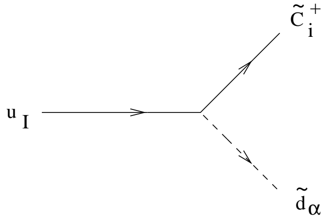
Figure 12: g_2 (V_{IJ}^{CKM}) (S_{DL}^{CKM})_J U_{i1} P_+ + \frac{g_2}{2m_W \cos} (V_{IJ}^{CKM}) (S_{DR}^{CKM})_J m_J^d U_{22} P_- + \frac{g_2}{2m_W \sin} (V_{IJ}^{CKM}) (S_{DL}^{CKM})_J m_I^u V_{i2} P_-
