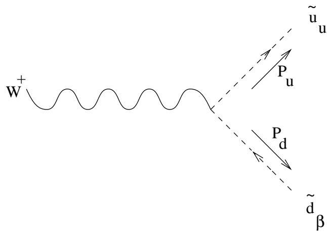
Figure 23: \frac{ig_2}{2} (P_d - P_u) F^1
