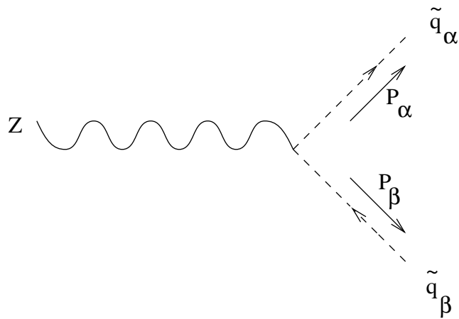
Figure 25: \frac{i g_2}{\cos w} F^{2I} (P_\alpha - P_\beta) (T_{3I} - q \sin^2 w)
