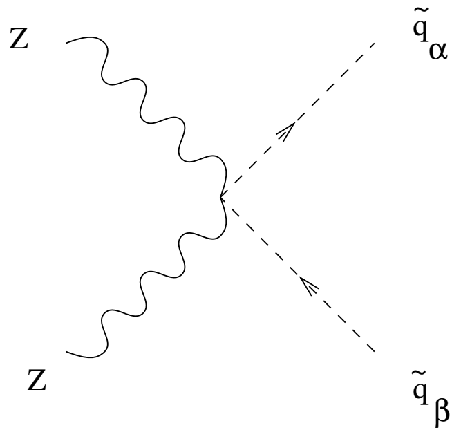
Figure 30: \frac{g^2}{\cos^2 \theta_w} F^{2I} (T_{3I} - q \sin^2 \theta_w)^2
