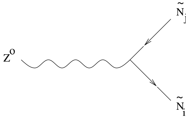
Figure 21: \frac{g}{\cos w} \bar{\psi} (O_{ij}^{\text{L}} P_L + O_{ij}^{\text{R}} P_R) \psi
