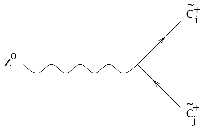
Figure 20: \frac{g_2}{\cos w} [O_{ij}^{(L)} P_L + O_{ij}^{(R)} P_R]
