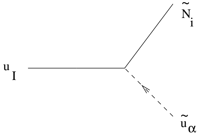
Figure 15: \frac{p_-}{2g_2 \tan w} \left( \frac{SCKM}{UL} \right)_I [T_{3I} N_{i2} \tan w (T_{3I} \epsilon) N_{i1}] \mathbb{P} + \frac{g_2 m_I^u}{2m_w \sin} (N_{i4} \left( \frac{SCKM}{UL} \right)_I \mathbb{P} + N_{i4} \left( \frac{SCKM}{UR} \right)_I \mathbb{P}_L :)
