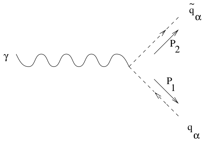
Figure 24: ie (P_1 - P_2)
