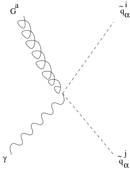
Figure 34: 2g_3 e e_q T_{ij}^a
