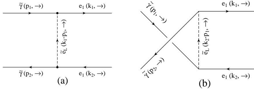
Figure 36: The annihilation of a pair of photinos into an electron-positron pair via a t-channel exchange of a left-handed scalar electron. The arrows on the lines label the direction of fermion number propagation. The arrows appearing together with the momenta label the direction of momentum flow.
