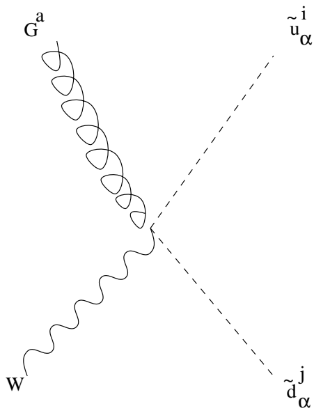
Figure 33: \frac{2}{3} g_2 g_s t_{ij}^a g F^1
