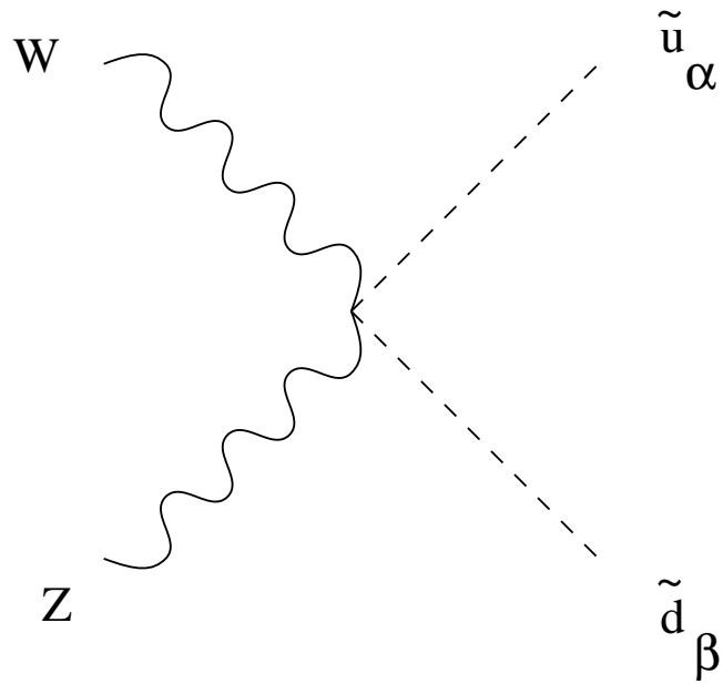
Figure 28: \frac{g_2^2 Y_Q \sin^2 w}{2 \cos w} F 1
