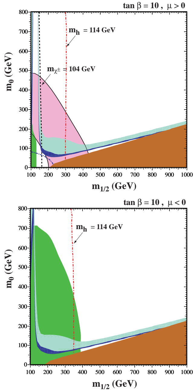
Figure 1: m SUGRA/CMSSM parameter space exclusion plots taken from [396], in which A_0 = 0 and other parameters are as shown. The darkest "V" shaped thin strip corresponds to the region with 0.094 < h^2 < 0.129 , while a bigger strip with a similar shape corresponds to the region with 0.1 < h^2 < 0.3 . (There are other dark strips as well when examined carefully.) The triangular region in the lower right hand corner is excluded by m_{\tilde{e}_1} < m_{\tilde{e}^0} , since DM cannot be charged and hence is a neutralino \tilde{e}^0 ). Other shadings and lines correspond to accelerator constraints. In the lower figure ( \mu < 0 ), most of the DM favored region below m_{1/2} < 400 GeV is ruled out by the b \rightarrow s constraint. In the upper figure, the medium shaded band encompassing the bulge region shows that the region favored by dark matter constraints is in concordance with the region favored by g_{\mu^2} measurements. The Higgs and chargino mass bounds are also as indicated: the parameter space left of
