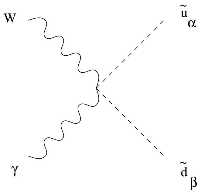
Figure 27: \frac{g_2 e}{2} Y_0 F^1
