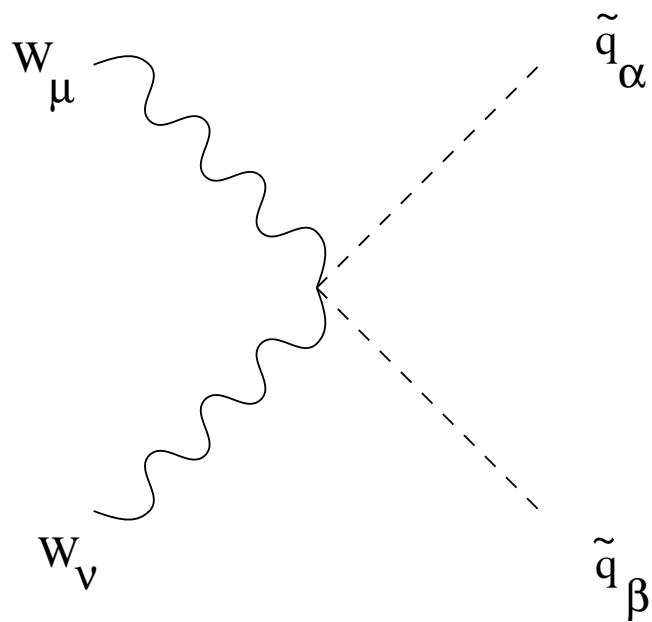
Figure 26: \frac{g_2^2}{2} \left( \begin{smallmatrix} \text{SCKM} \\ \text{qL} \end{smallmatrix} \right)_I \left( \begin{smallmatrix} \text{SCKM} \\ \text{qL} \end{smallmatrix} \right)_I
