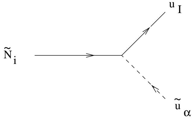
Figure 14: \frac{p_-}{2g_2 \tan w} \left( \frac{SCKM}{UL} \right)_I [T_{3I} N_{i2} \tan w (T_{3I} \epsilon) N_{i1}] \mathbb{P} + \frac{g_2 m_I^u}{2m_w \sin} (N_{i4} \left( \frac{SCKM}{UL} \right)_I \mathbb{P} + N_{i4} \left( \frac{SCKM}{UR} \right)_I \mathbb{P}_R :)
