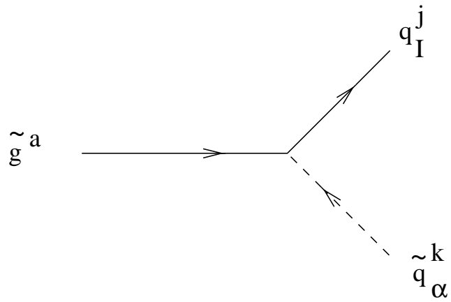
Figure 16: \bar{p} \frac{1}{2g_3} T^a_{jk} G^{-1} \left( \frac{SCKM}{q_L} \right)_I P_R G \left( \frac{SCKM}{q_R} \right)_I P_L
