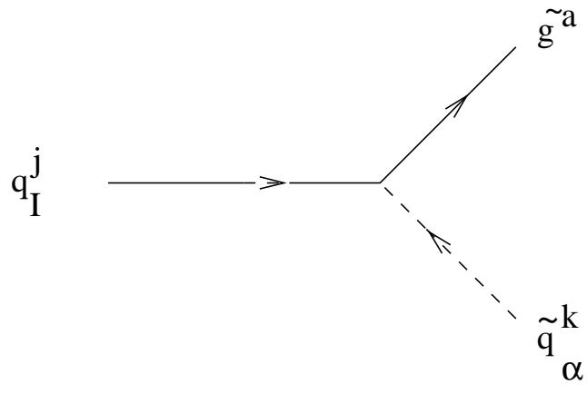
Figure 17: \bar{p} \frac{1}{2g_3} T^a_{kj} (G \left( \frac{SCKM}{q_L} \right)_I P_L G^{-1} \left( \frac{SCKM}{q_R} \right)_I P_R)
