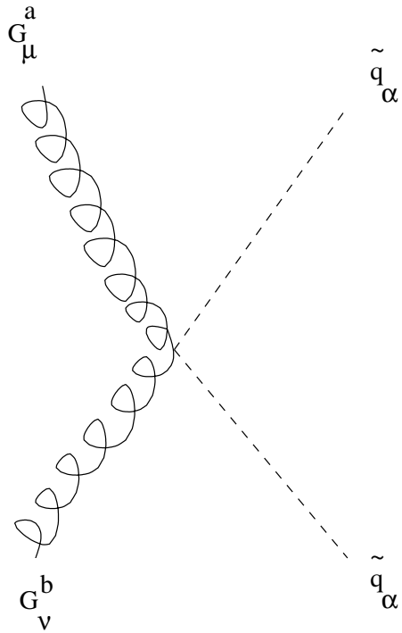
Figure 32: g_3^2 (\frac{1}{3} \delta_{ab} 1 + d_{abc} T^c) g
