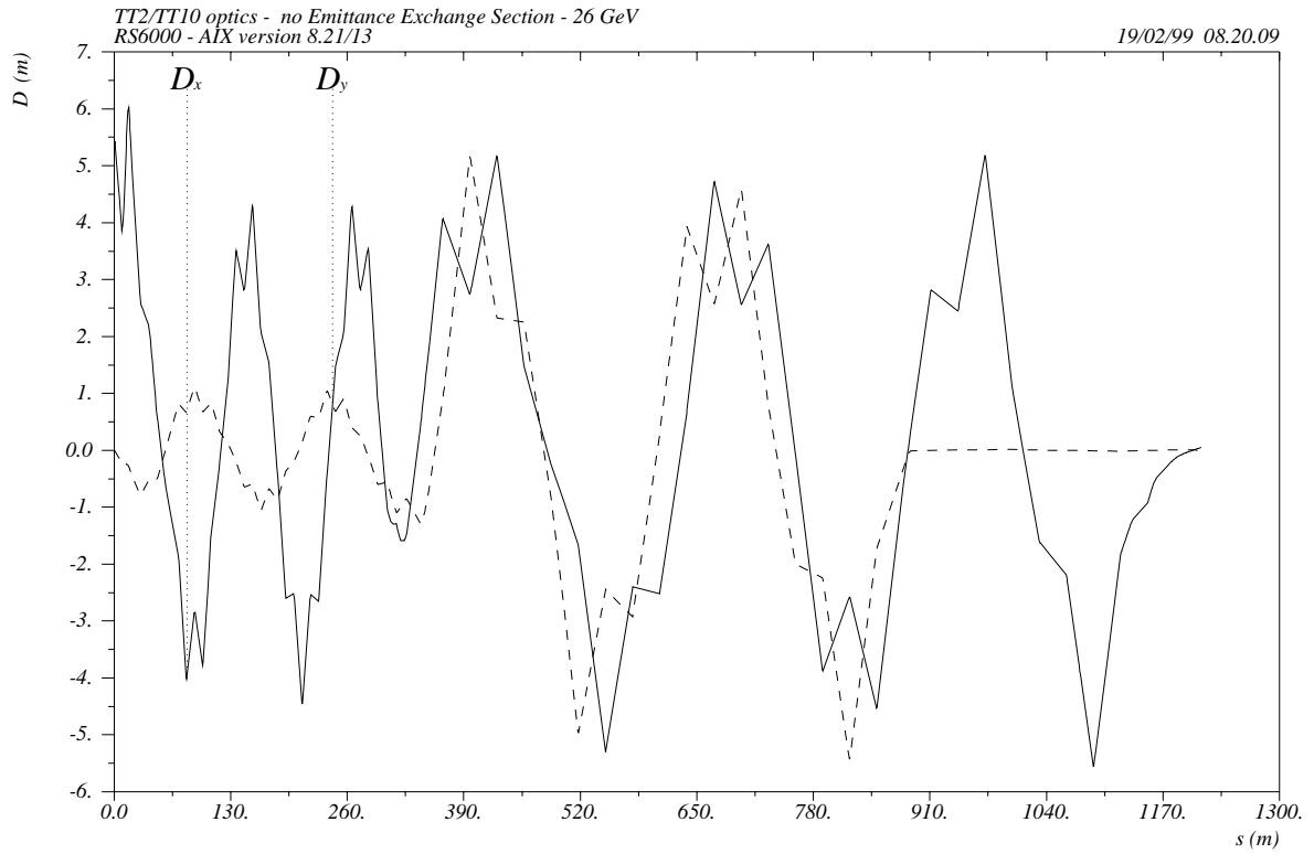
Figure 6: Horizontal and vertical dispersion in TT2/TT10 for the matched optics as computed by MAD.
