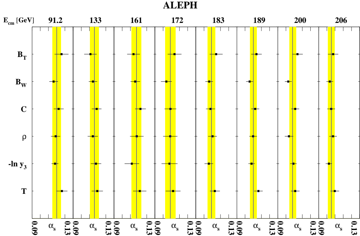
Figure 12: Summary of all individual measurements of \alpha_s using six variables at eight centre-of-mass energies. The error bars correspond to the total uncertainties, the shaded areas to the combined measurements given in Table 7.
