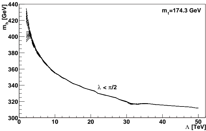
Fig.1. The upper bound on the Higgs boson mass from the standard triviality condition T1: \lambda < \pi/2 (the small-scale structure is due to numerical inaccuracies).
