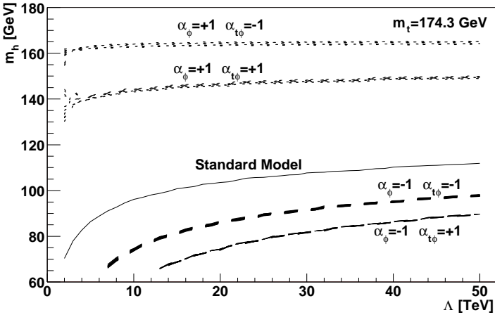
Fig. 2. Lower bounds on the Higgs boson mass (all the S's conditions satisfied), the black curve represents the SM limit, the upper (dotted) curves are for \alpha_\phi > 0 , and the lower (dashed) ones for \alpha_\phi < 0 . For each style the higher branches correspond to \alpha_{t\phi} < 0 while lower for \alpha_{t\phi} > 0 .
