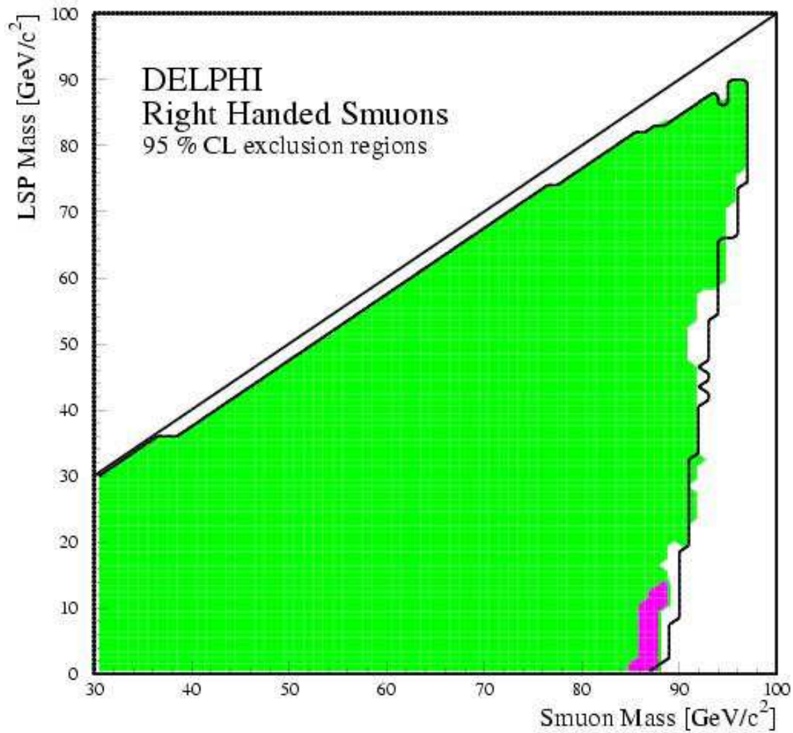
Figure 16: Excluded region in the (M_{\tilde{\mu}_R}, M_{LSP}) plane. The shaded region shows the obtained limit. The lighter shaded region is excluded taking the branching ratios for each mass point with the SUSY parameters \tan \beta=1.5 and \mu=-200 \text{ GeV}/c^2 . The solid line shows the corresponding expected limit. If the branching ratio of \tilde{\mu} \rightarrow \mu\chi_1^0 is set to 1, the darker shaded region is also excluded (for a discussion on the low smuon mass region see section 6.3).
