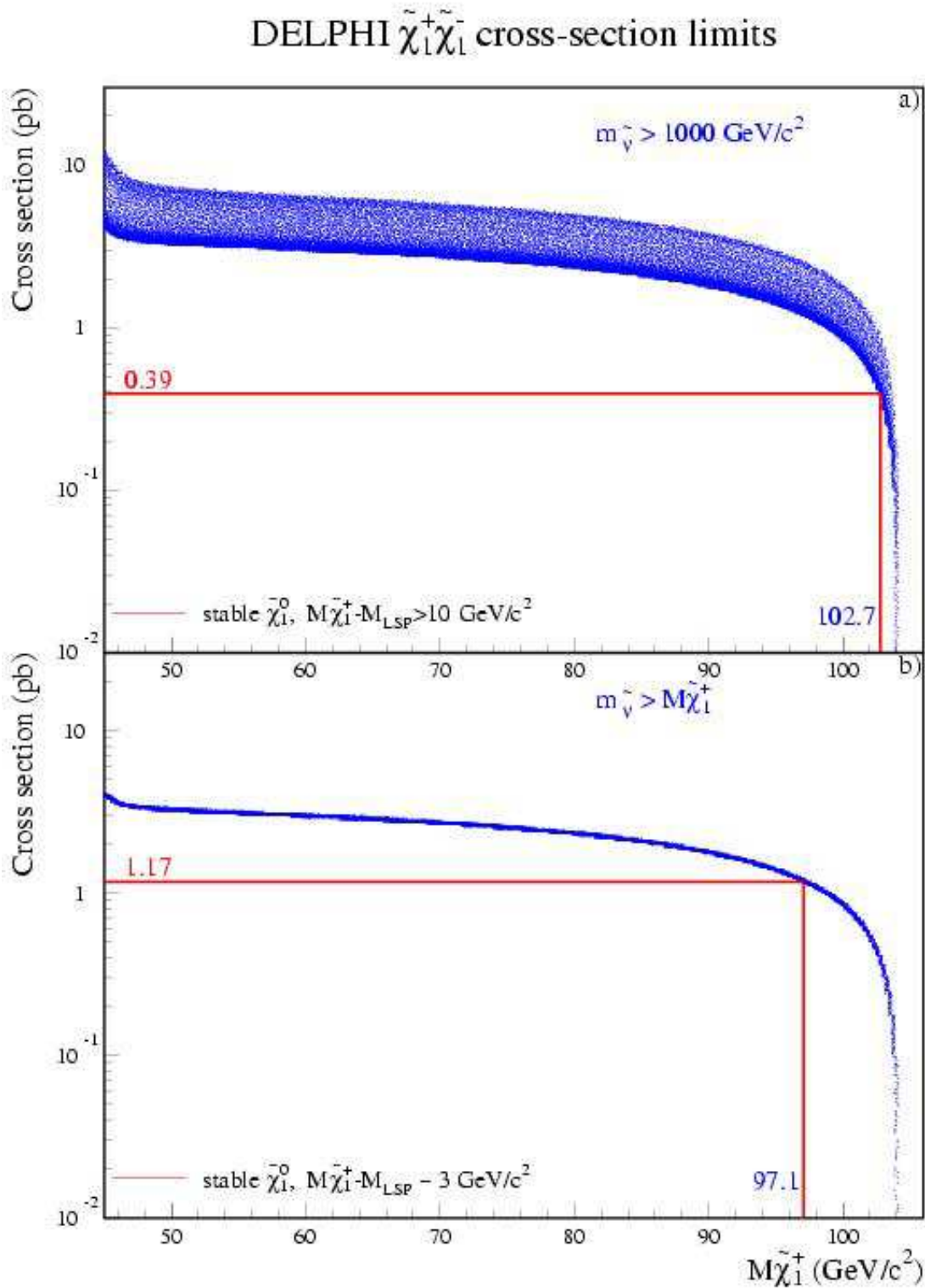
Figure 28: Expected cross-sections in pb at 208 GeV (dots) versus the chargino mass in a) for \Delta M > 10 \text{ GeV}/c^2 and b) for \Delta M \sim 3 \text{ GeV}/c^2 . The spread in the dots originates from the random scan over the parameters \mu and M_2 . A heavy sneutrino ( m_{\tilde{\nu}} > 1000 \text{ GeV}/c^2 ) has been assumed in a) and m_{\tilde{\nu}} > M_{\tilde{\chi}_1^\pm} in b). The minimal cross-sections below the mass limits are indicated by the horizontal lines.
