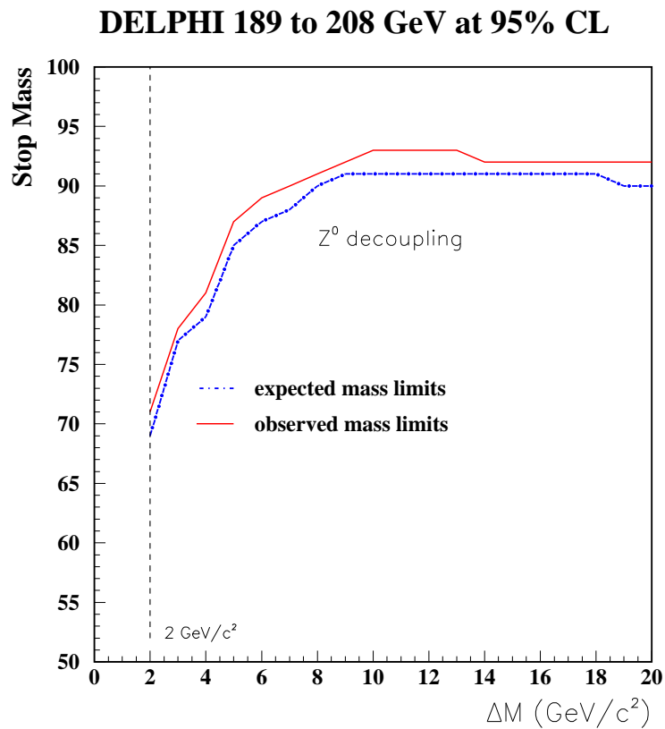
Figure 25: Stop mass limit as a function of \Delta M for a purely left-handed stop and for the stop mixing angle which minimises the cross-section.
