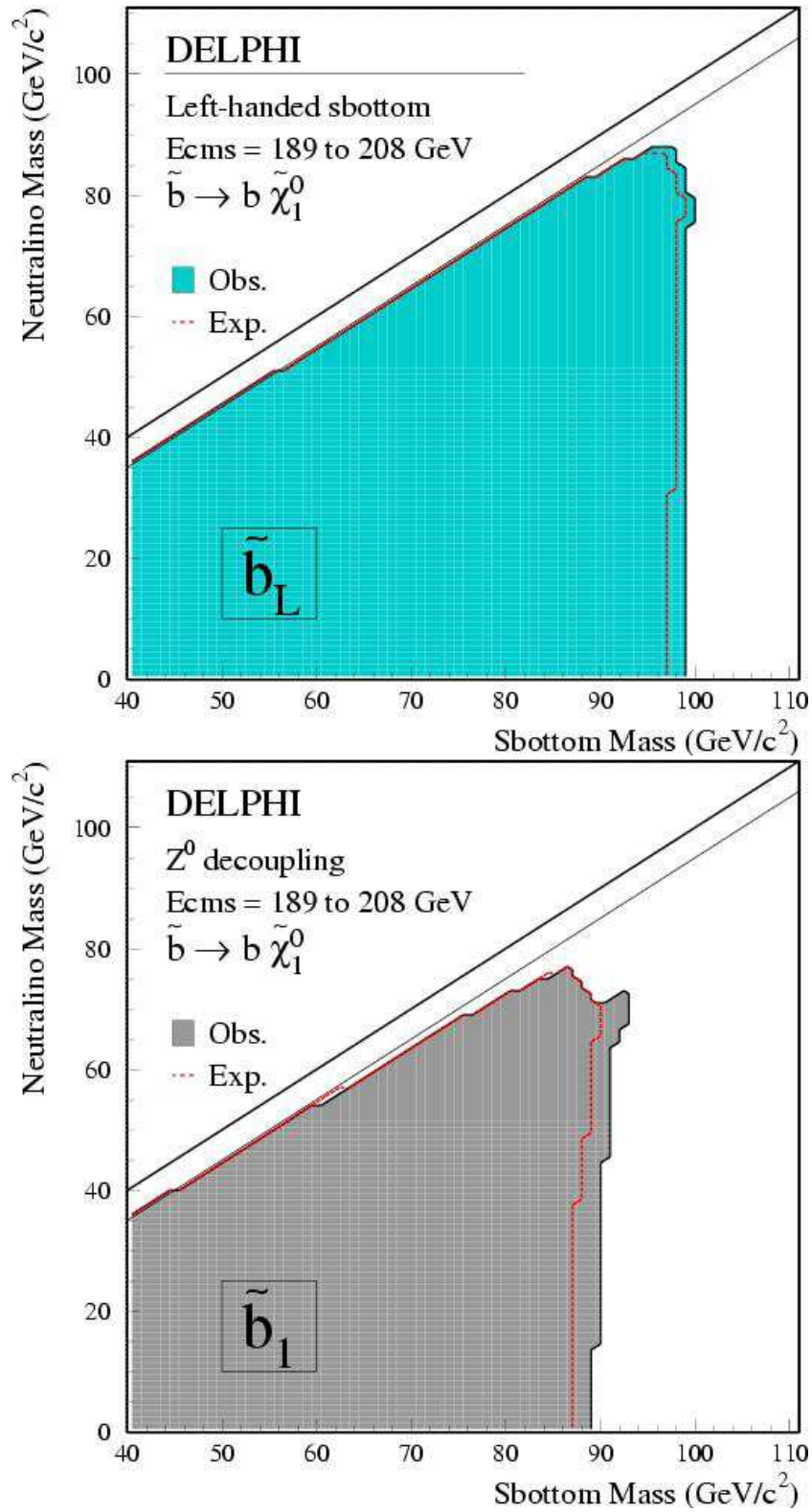
Figure 24: Excluded regions at for the sbottom search in the plane (M_{\tilde{b}_1}, M_{\tilde{\chi}_1^0}) for purely left handed sbottoms (top) and for the states at the Z decoupling (bottom). The shaded areas show the observed excluded regions and the lines correspond to the expected exclusions (for a discussion on the low sbottom mass region see section 6.3).
