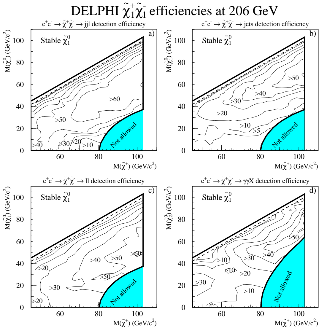
Figure 26: Chargino pair-production detection efficiencies (%) for the four decay channels a) jj\ell , b) jets , c) \ell\ell and d) rad , at 206 GeV in the (M_{\tilde{\chi}^\pm}, M_{\tilde{\chi}_1^0}) plane. TPC sector 6 is on and a stable \tilde{\chi}_1^0 is assumed. The shaded areas are disallowed in the MSSM scheme.
