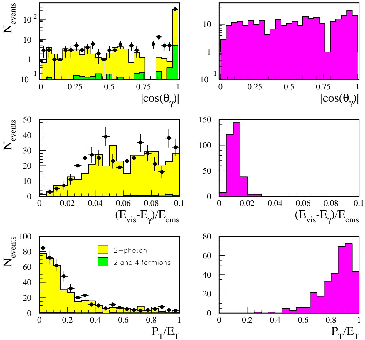
Figure 9: Some of the variables used in the selection for mass-degenerate charginos with an ISR photon tag. In the plots on the left the data (dots) are compared with the SM expectations. On the right, as an example, the corresponding distributions (with arbitrary normalisation) are shown for the signal with M(\tilde{\chi}_1^\pm) = 80 \text{ GeV}/c^2 and \Delta M = 1 \text{ GeV}/c^2 .
