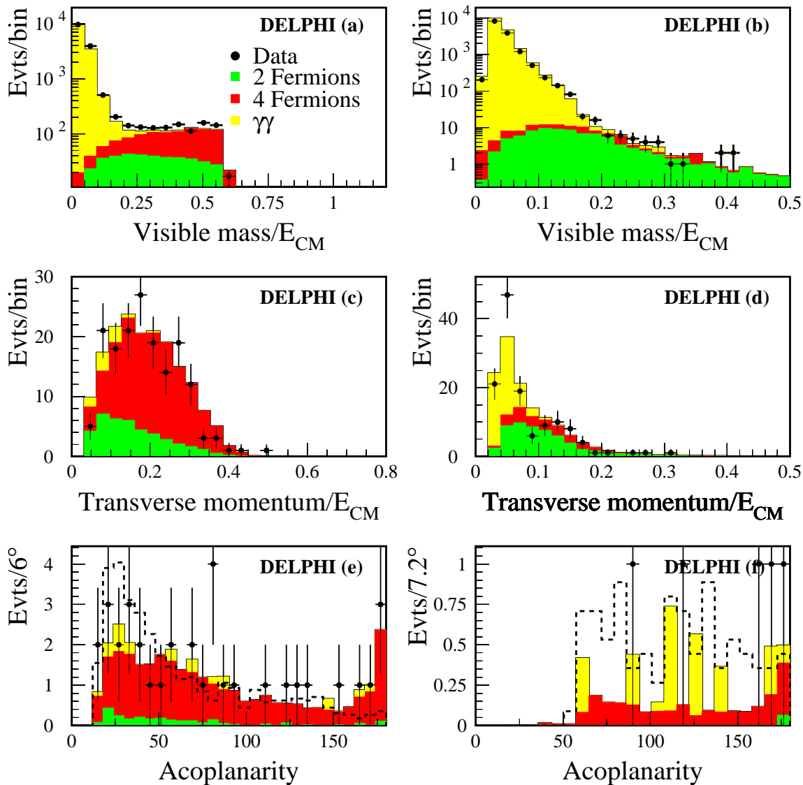
Figure 14: Comparison of real data from 2000 ( \sqrt{s} in the range 204–208 GeV) and simulation for the neutralino multilepton search (a,c,e) and asymmetric tau search (b,d,f), at the preselection (a,b), intermediate (c,d), and final selection (e,f) stages. The dashed line in (e) shows the multilepton signal expected for \tilde{\chi}_3^0\tilde{\chi}_2^0 production with \tilde{\chi}_3^0 \rightarrow \tilde{\chi}_2^0\ell^+\ell^- and \tilde{\chi}_2^0 decaying to \tilde{\chi}_1^0\ell^+\ell^- where M_{\tilde{\chi}_3^0}=103 GeV/ c^2 , M_{\tilde{\chi}_2^0}=51 GeV/ c^2 and M_{\tilde{\chi}_1^0}=45 GeV/ c^2 . In (f) the dashed line shows the tau cascade signal for \tilde{\chi}_2^0\tilde{\chi}_1^0 production with \tilde{\chi}_2^0 \rightarrow \tilde{\tau}\tau and \tilde{\tau} \rightarrow \tilde{\chi}_1^0\tau where M_{\tilde{\chi}_2^0}=75 GeV/ c^2 , M_{\tilde{\tau}}=44 GeV/ c^2 and M_{\tilde{\chi}_1^0}=37.5 GeV/ c^2 . The signals are normalised to a cross-section of 0.4 pb.
