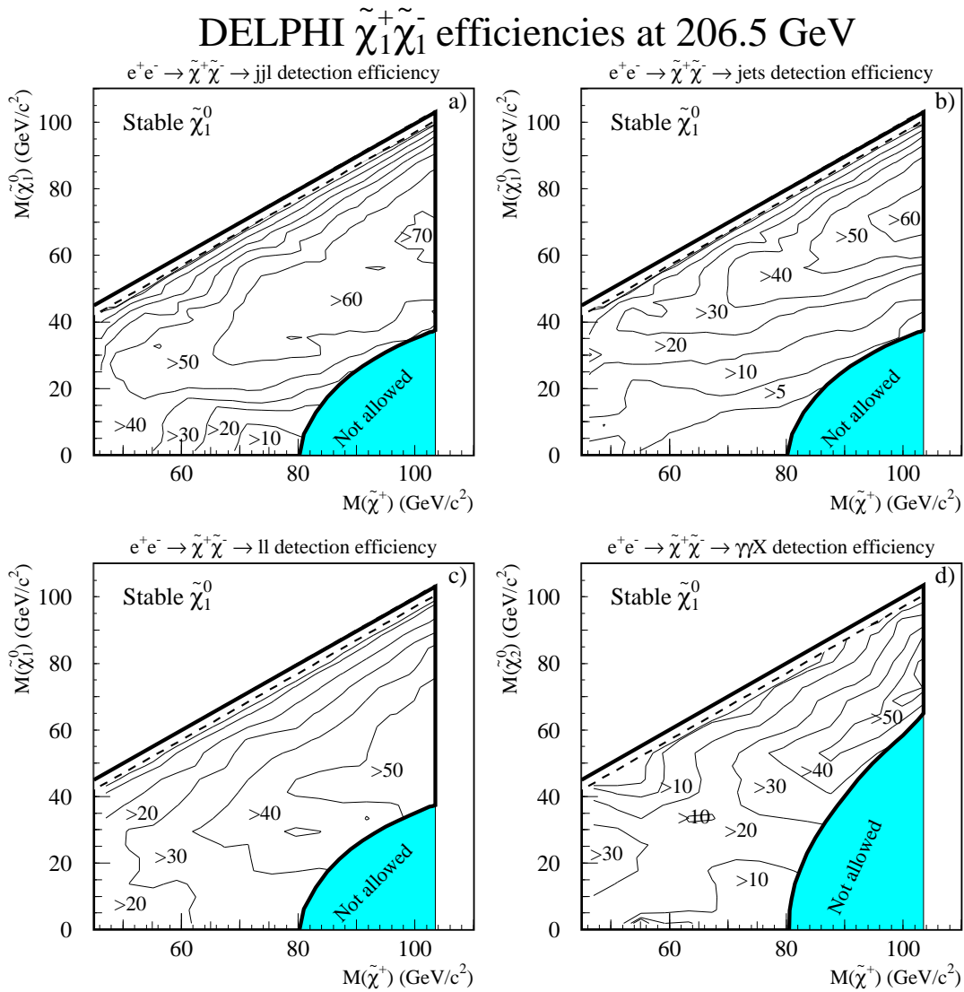
Figure 27: Chargino pair-production detection efficiencies (%) for the four decay channels a) jj\ell , b) jets , c) \ell\ell and d) rad , at 206.5 GeV in the (M_{\tilde{\chi}^\pm}, M_{\tilde{\chi}^0}) plane. TPC sector 6 is off and a stable \tilde{\chi}_1^0 is assumed. The shaded areas are disallowed in the MSSM scheme.
