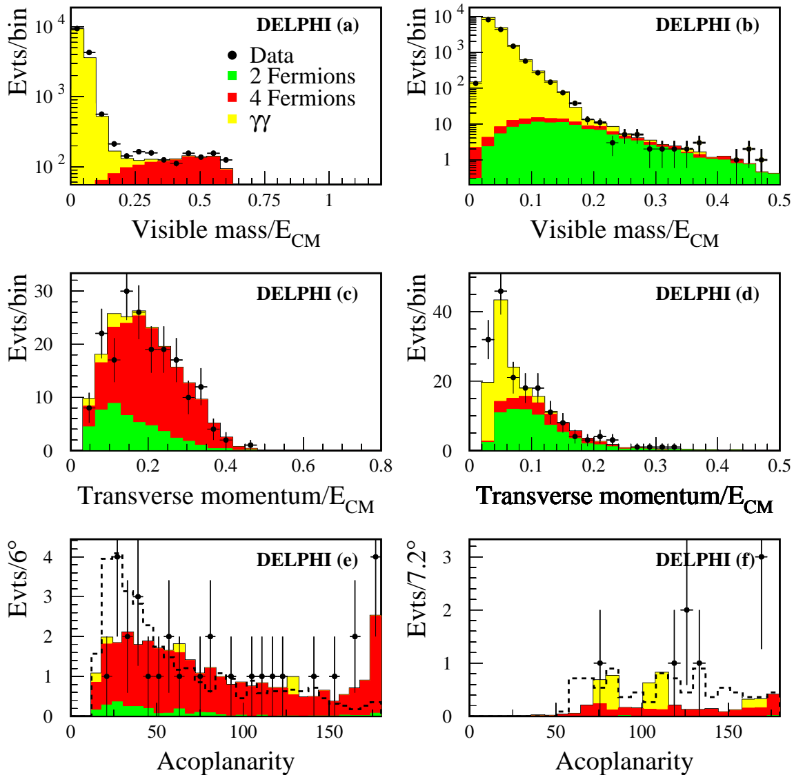
Figure 13: Comparison of real data from 1999 ( \sqrt{s} in the range 192–202 GeV) and simulation for the neutralino multilepton search (a,c,e) and asymmetric tau search (b,d,f), at the preselection (a,b), intermediate (c,d), and final selection (e,f) stages. The dashed line in (e) shows the multilepton signal expected for \tilde{\chi}_3^0\tilde{\chi}_2^0 production with \tilde{\chi}_3^0 \rightarrow \tilde{\chi}_2^0\ell^+\ell^- and \tilde{\chi}_2^0 decaying to \tilde{\chi}_1^0\ell^+\ell^- where M_{\tilde{\chi}_3^0}=103 GeV/ c^2 , M_{\tilde{\chi}_2^0}=51 GeV/ c^2 and M_{\tilde{\chi}_1^0}=45 GeV/ c^2 . In (f) the dashed line shows the tau cascade signal for \tilde{\chi}_2^0\tilde{\chi}_1^0 production with \tilde{\chi}_2^0 \rightarrow \tilde{\tau}\tau and \tilde{\tau} \rightarrow \tilde{\chi}_1^0\tau where M_{\tilde{\chi}_2^0}=75 GeV/ c^2 , M_{\tilde{\tau}}=44 GeV/ c^2 and M_{\tilde{\chi}_1^0}=37.5 GeV/ c^2 . The signals are normalised to a cross-section of 0.4 pb.
