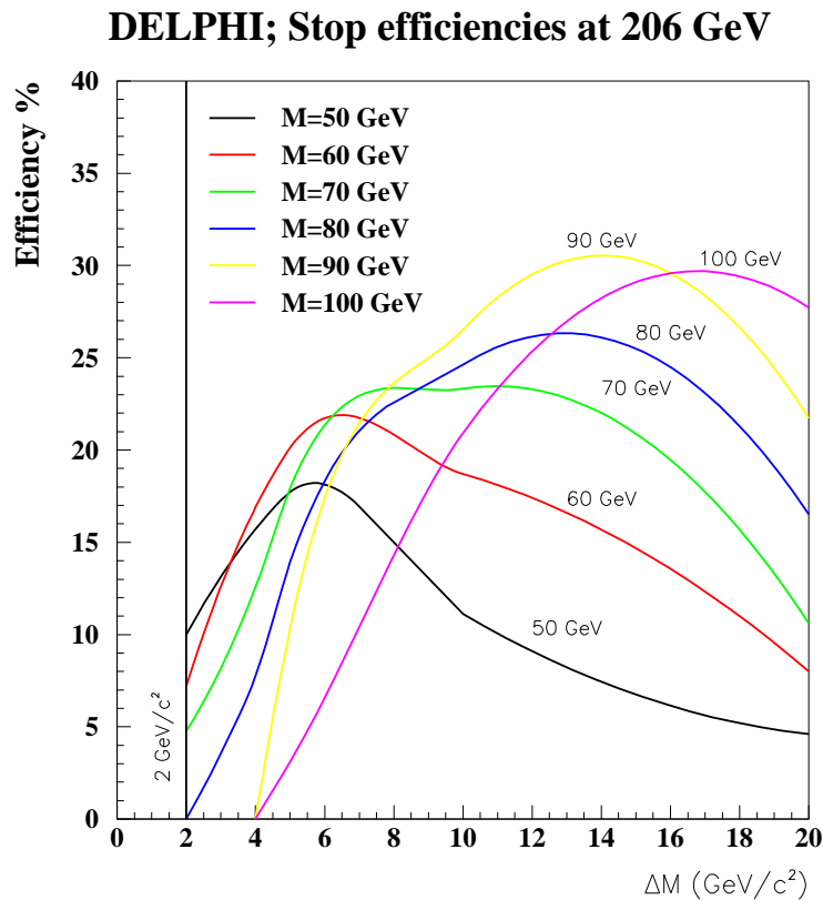
Figure 22: Signal efficiency of the stop search in the nearly degenerate scenario for different mass hypothesis as a function of \Delta M = M_{\tilde{t}_1} - M_{\tilde{\chi}_1^0} , for \sqrt{s}=189 and 206 GeV.
