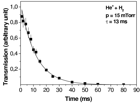
Fig. 12. Lifetime measurement: transmission as a function of t_{cool} for {}^4\text{He}^+ . The line corresponds to an exponential decay fit with a time constant of 13 ms. Here, the \text{H}_2 pressure is 15 mTorr.
