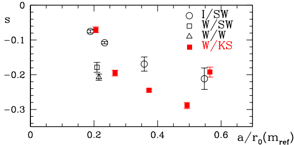
Figure 1. Lattice spacing dependence of slopes s .
