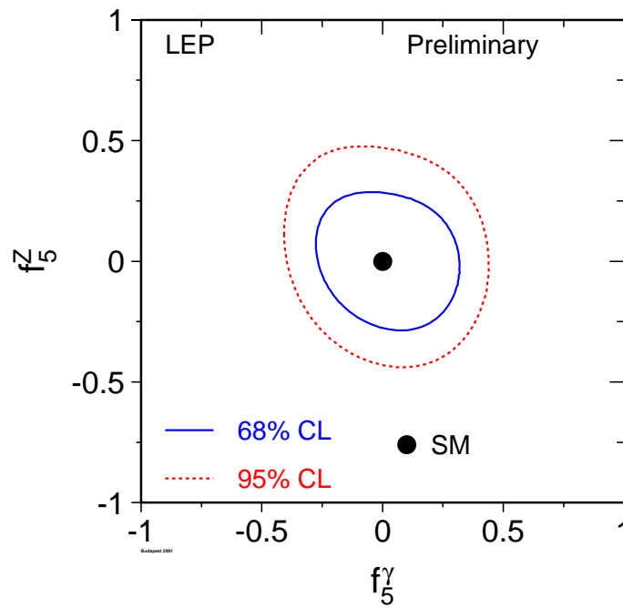
Figure 8: Contour curves of 68% C.L. and 95% C.L. in the plane (f_4^\gamma, f_4^Z) and (f_5^\gamma, f_5^Z) showing the LEP combined result.
