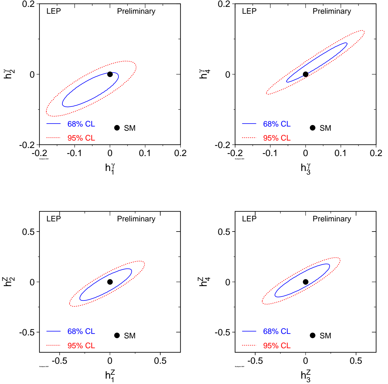
Figure 6: Contour curves of 68% C.L. and 95% C.L. in the planes (h_1^\gamma, h_2^\gamma) , (h_3^\gamma, h_4^\gamma) , (h_1^Z, h_2^Z) and (h_3^Z, h_4^Z) showing the LEP combined result.
