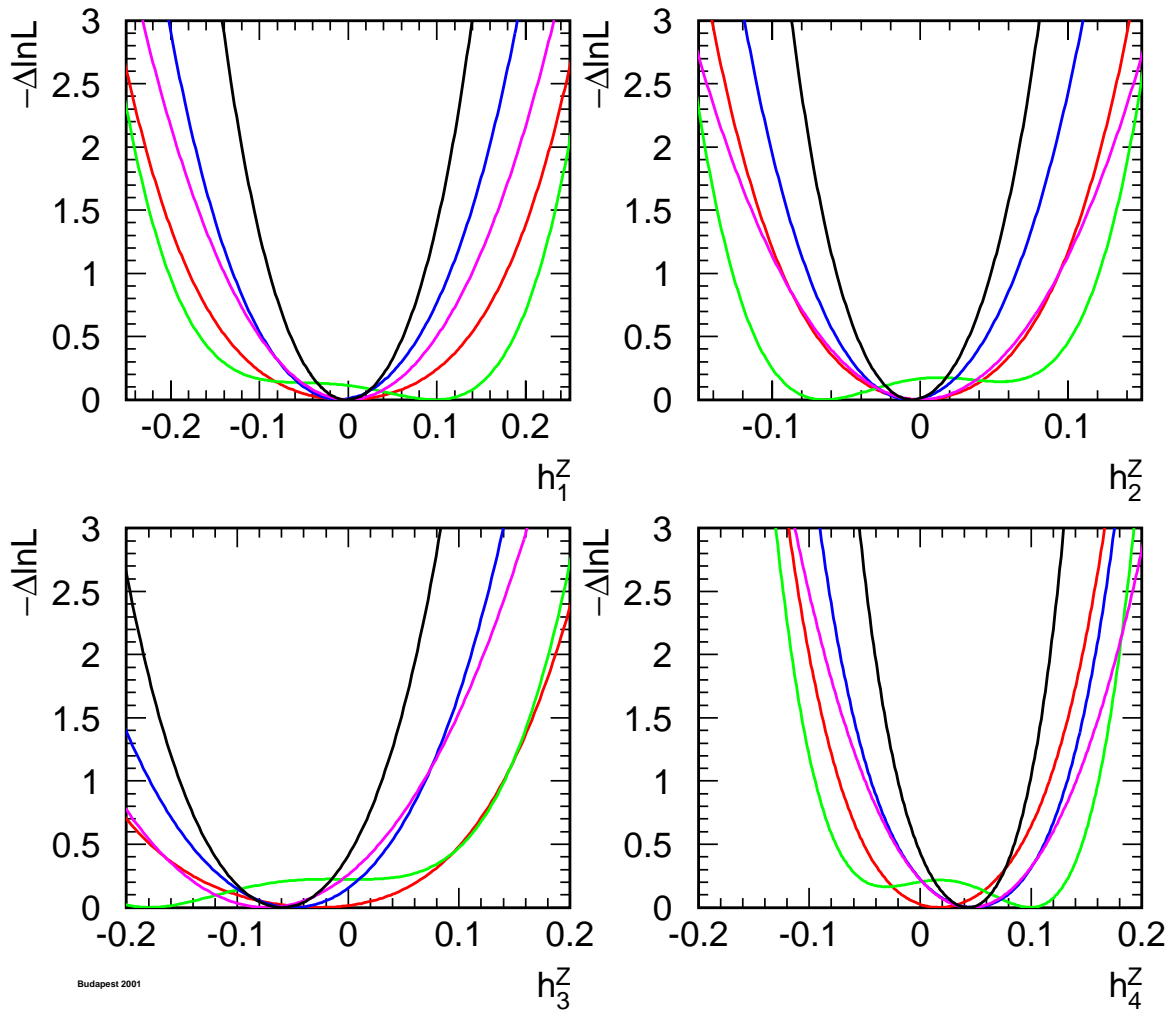
Figure 5: The \log \mathcal{L} curves of the four experiments, and the LEP combined curve for the four neutral TGCs h_i^Z , i = 1, 2, 3, 4 . In each case, the minimal value is subtracted.
