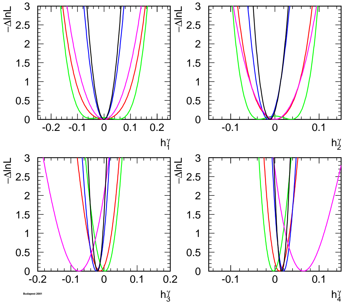
Figure 4: The log \mathcal{L} curves of the four experiments, and the LEP combined curve for the four neutral TGCs h_i^\gamma , i = 1, 2, 3, 4 . In each case, the minimal value is subtracted.
