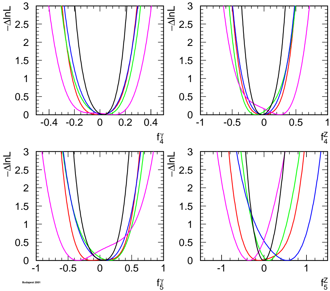
Figure 7: The log \mathcal{L} curves of the four experiments, and the LEP combined curve for the four neutral TGCs f_i^V , V = \gamma, Z , i = 4, 5 . In each case, the minimal value is subtracted.
