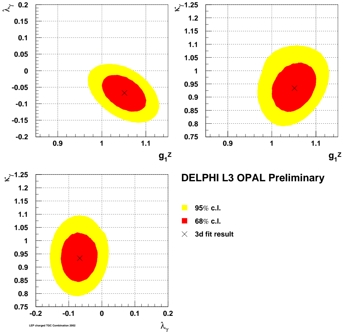
Figure 3: The result of the three-parameter fit, plotted in the two-dimensional planes of the three TGC pairs, with the third TGC parameter at the fitted value. In each plane, the respective 68% and 95% two-parameter confidence level contours are shown. The fitted coupling value is indicated with a cross; the Standard Model value for each fit is in the center of the grid. The contours include the contribution from systematic uncertainties, and data from DELPHI, L3 and OPAL.
