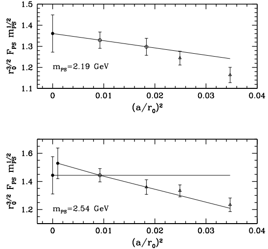
Figure 1. Continuum extrapolation of the decay constant F_{\text{PS}}\sqrt{m_{\text{PS}}} at two meson masses from two resp. one lattice.
