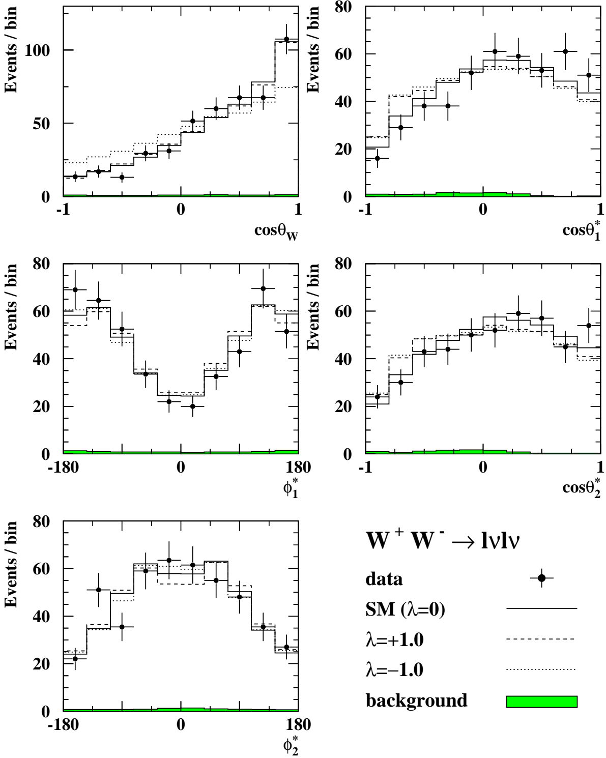
Figure 4: Distributions of the kinematic variables \cos\theta_W , \cos\theta_1^* , \phi_1^* , \cos\theta_2^* and \phi_2^* in the \ell\bar{\nu}_\ell\ell\nu_\ell analysis, where \cos\theta_1^* , \phi_1^* ( \cos\theta_2^* , \phi_2^* ) are the decay angles of the charged lepton (anti-lepton) from the W^- ( W^+ ) in the parent W rest frame. All events enter with a total weight of one, but in the case of events with two ambiguous solutions, each solution enters with a weight of 0.5. The histograms, normalized to the number of data events, show the expectation of the Standard Model and the cases of \lambda = \pm 1 . The shaded histograms represent the contribution of the background.
