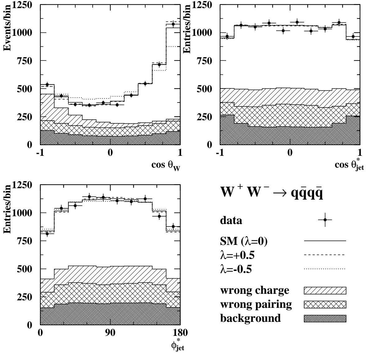
Figure 3: Distribution of the kinematic variables \cos \theta_W , \cos \theta_{jet}^* , and \phi_{jet}^* for q\bar{q}q\bar{q} events. In the \cos \theta_{jet}^* , and \phi_{jet}^* distributions there are two entries per event. The solid points represent the data. The histograms show the Monte Carlo expectation of the Standard Model (solid line) and the cases of \lambda=+0.5 and \lambda=-0.5 (dashed and dotted lines respectively). The Monte Carlo histograms are normalised to the number of data events. The open histograms show the contribution from correct pairing and correct charge assignment. The single hatched histograms represent the contribution from correct pairing, but wrong charge assignment. The cross-hatched histograms correspond to the contribution from wrong pairing, and the dark histograms show the contribution of background.
