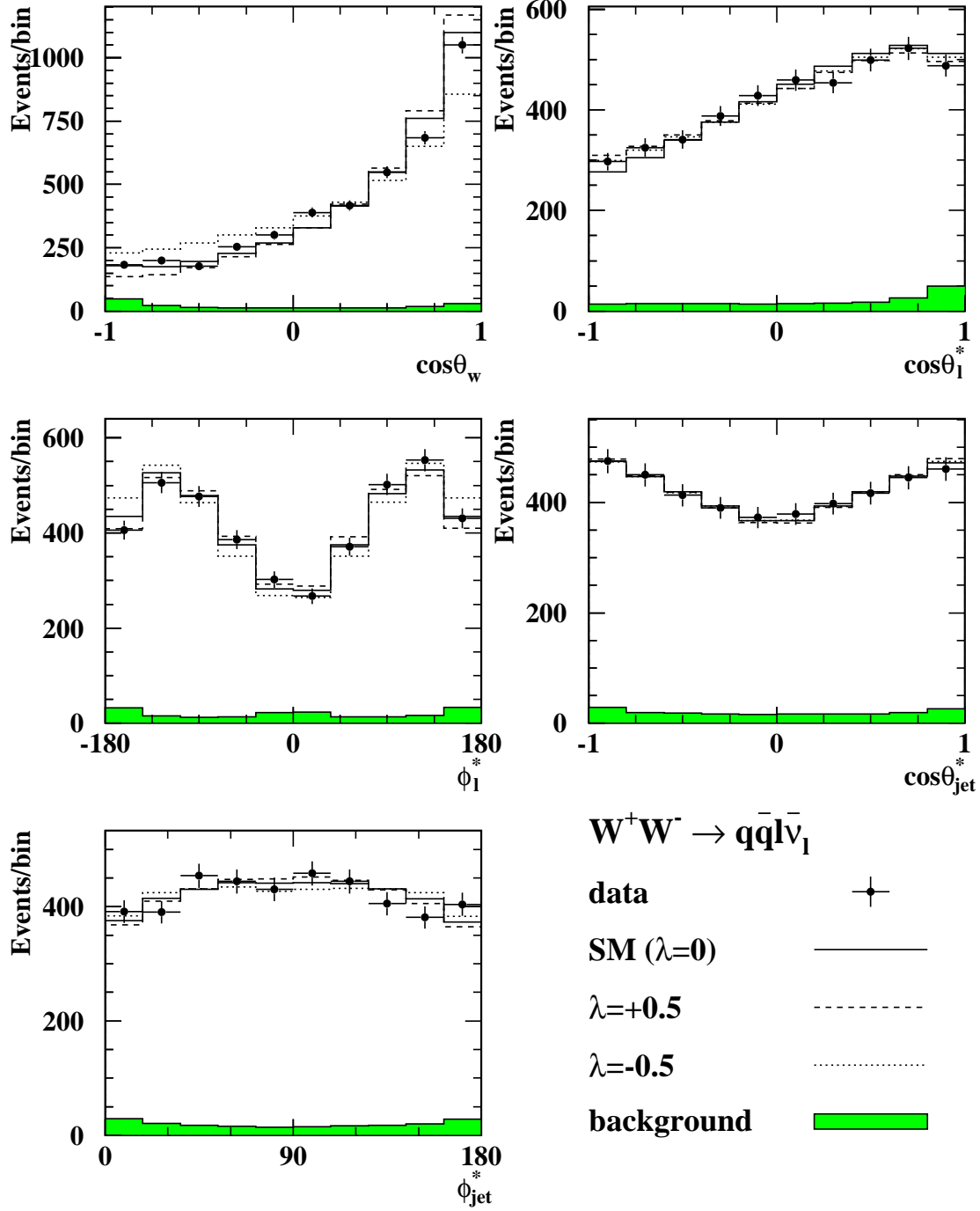
Figure 1: Distributions of the kinematic variables \cos\theta_W , \cos\theta_\ell^* , \phi_\ell^* , \cos\theta_{\text{jet}}^* and \phi_{\text{jet}}^* , obtained from the q\bar{q}l\nu_{\bar{l}} candidates. The solid points represent the data. The histograms show the Monte Carlo expectation of the Standard Model (solid line) and the cases of \lambda = +0.5 and \lambda = -0.5 (dashed and dotted lines respectively). The Monte Carlo histograms are normalised to the number of data events. The shaded histograms show the non- q\bar{q}l\nu_{\bar{l}} background. In the case of W^+ \rightarrow \bar{l}\nu decays the value of \phi_\ell^* is shifted by 180^\circ in order to overlay W^+ and W^- distributions in the same plot, which is valid so long as CP is conserved.
