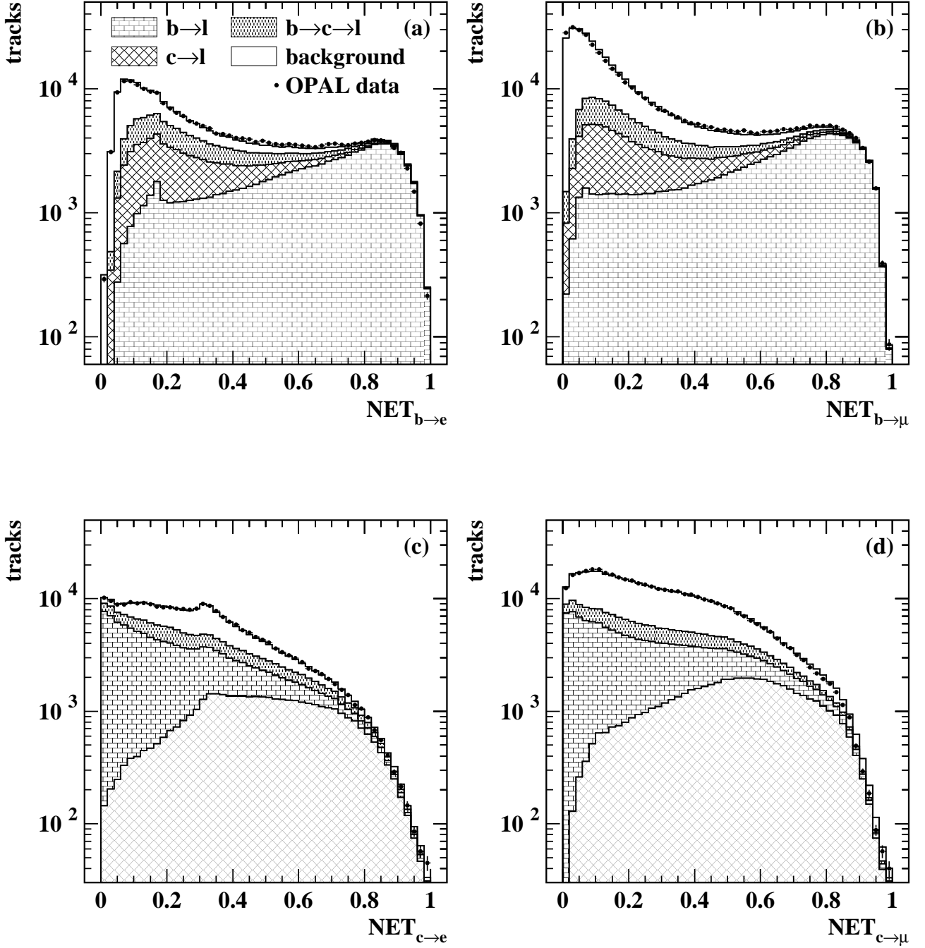
Figure 1: Outputs of the neural networks designed to select (a) b \rightarrow e , (b) b \rightarrow \mu , (c) c \rightarrow e and (d) c \rightarrow \mu decays. The data are shown by the points with error bars, and the expected contributions from different lepton sources by the hatched histograms.
