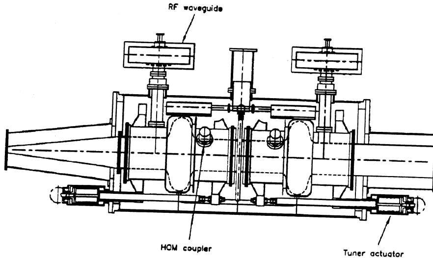
Fig. 2: Schematic layout of sc mono-cell cavities for the Large Hadron Collider LHC.
