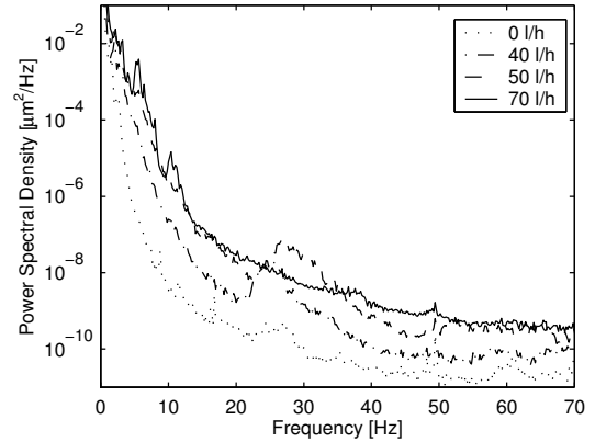
Figure 9: Power spectral density of vertical displacement as measured on the doublet mounted on the air pressure stabilization system.
