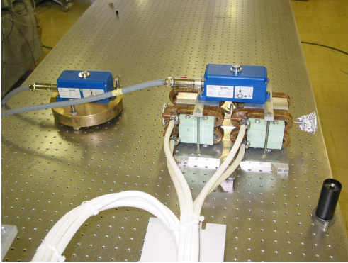
Figure 3: Detail of the installation of the doublet used for the measurements. The doublet is fixed on top of the honeycomb table described in [9], which is mounted on a stabilization device. The white cables feed the cooling circuit inside the magnet coils.
