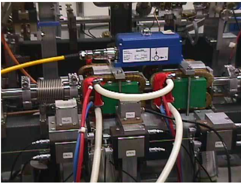
Figure 11: Sensor installation for the in-situ measurements of quadrupole vibrations in the CTF2 site.
