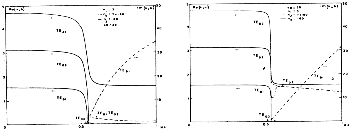
Fig. 7 Plots of Re(k_x b) and Im(k_x b) for TE_{01} , TE_{02} , TE_{03} modes versus kb for a waveguide with kb = 20 (fig.7a) and kb = 150 (fig.7b). In both cases n_1 = 3 and \tilde{n}_2 = i60 (—) and \tilde{n}_2 = 7 + i60 (---).
