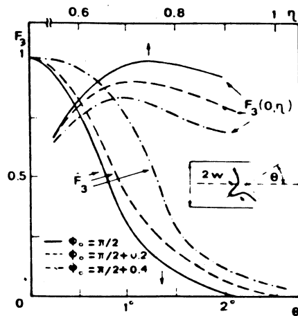
Fig. 9 Coupling efficiency F_3(0, \eta) of a cylindrical gaussian beam versus \eta = w/b and F_3 = F_3(\theta, \eta_{\text{opt}})/F_3(0, \eta_{\text{opt}}) for different values of \Phi_0 . \theta is the angle between the waveguide and the laser beam axis. Note that the dielectric coating decrease the sensitivity of the coupling efficiency to the alignment.
