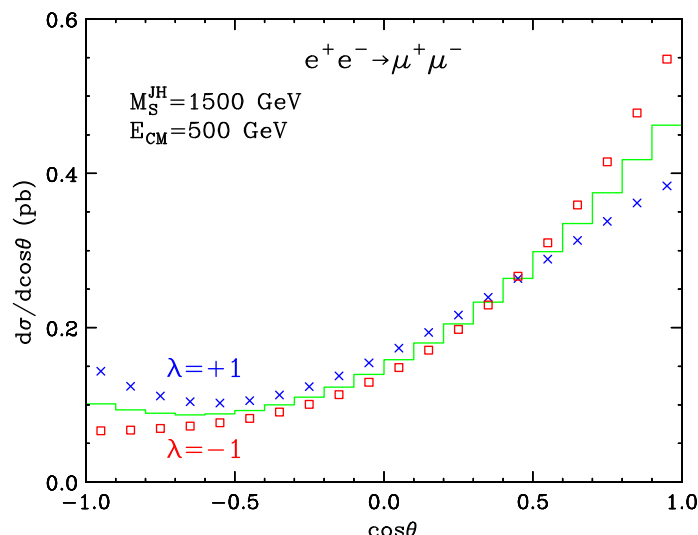
Figure 3: The AMEGIC++ result for e^+e^- \rightarrow \mu^+\mu^- , for centre-of-mass energy E_{CM} = 500 \text{ GeV} , M_S^{JH} = 1500 \text{ GeV} , and \lambda = +1 (crosses) or \lambda = -1 (squares). The solid histogram is the pure Standard Model result.
