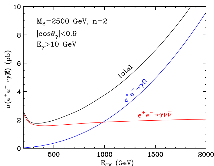
Figure 4: The total cross-section for e^+e^- \rightarrow \gamma G as a function of the centre-of-mass energy E_{CM} , for M_S = 2500 \text{ GeV} , n = 2 and photon energy and angular acceptance cuts of E_\gamma > 10 \text{ GeV} and |\cos\theta_\gamma| < 0.9 , respectively. Compare with figure 3 of [10].
