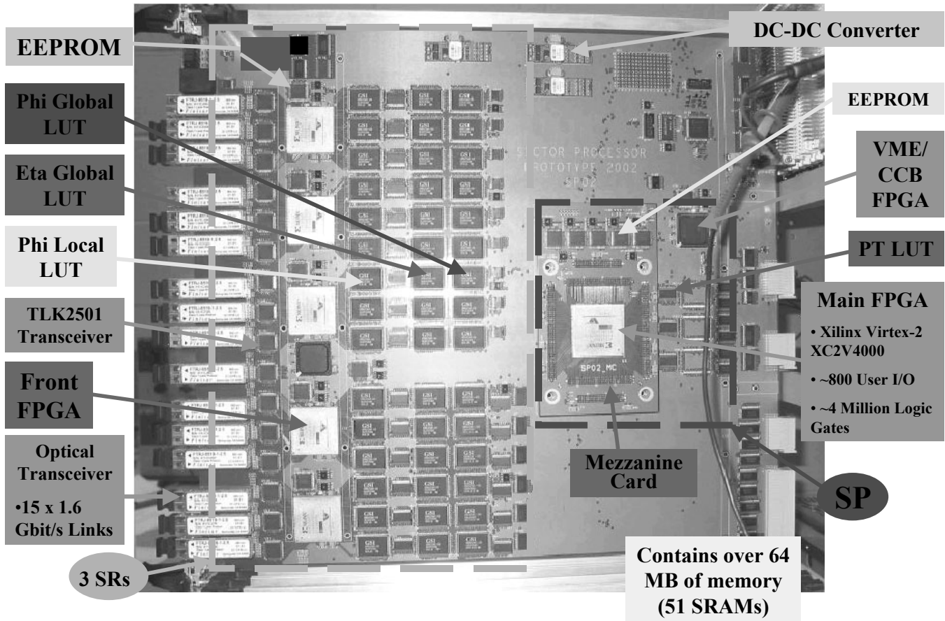
Figure 3: Second Sector Processor prototype
