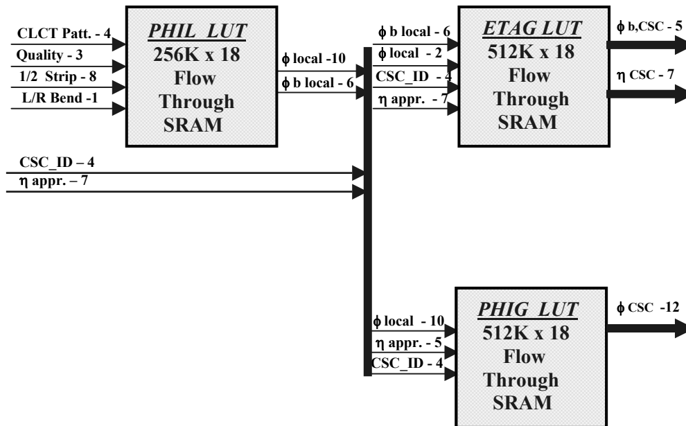
Figure 4: Sector Receiver look-up memory scheme. Here “CLCT Patt”, “Quality”, “½ Strip”, “L/R Bend”, “CSC_ID”, and “η appr.” are variables that describe a LCT received by the Sector Receiver. From this data, \phi with respect to the given chamber (“ \phi local”), and the bend angle (“ \phi b local”) are found. These are then sent to more memories from which \phi (“ \phi CSC-12”) and \eta (“ \eta CSC-7”) are reported.
