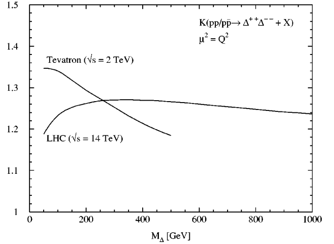
FIG. 2. K factors of doubly charged Higgs boson pair production at the Tevatron and the LHC. The parameters are the same as in Fig. 1. The curve for the Tevatron has been truncated at M_{\Delta} = 500 GeV, because the cross section is too small above and thus phenomenologically irrelevant.
