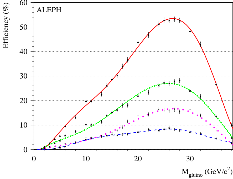
Figure 5: The q\bar{q}g\bar{g} selection efficiency as a function of the gluino mass, when P_{\bar{g}g} = 0\% , for the q\bar{q}R^0R^0 final state (dashed curve), the q\bar{q}R^\pm R^0 final state (dot-dashed curve), the q\bar{q}R^\pm R^\pm final state (dotted curve), and the sum of the three (full curve). The markers with error bars indicate the efficiencies obtained with each of the simulated samples, and the curves are obtained with a polynomial fit through these points.
