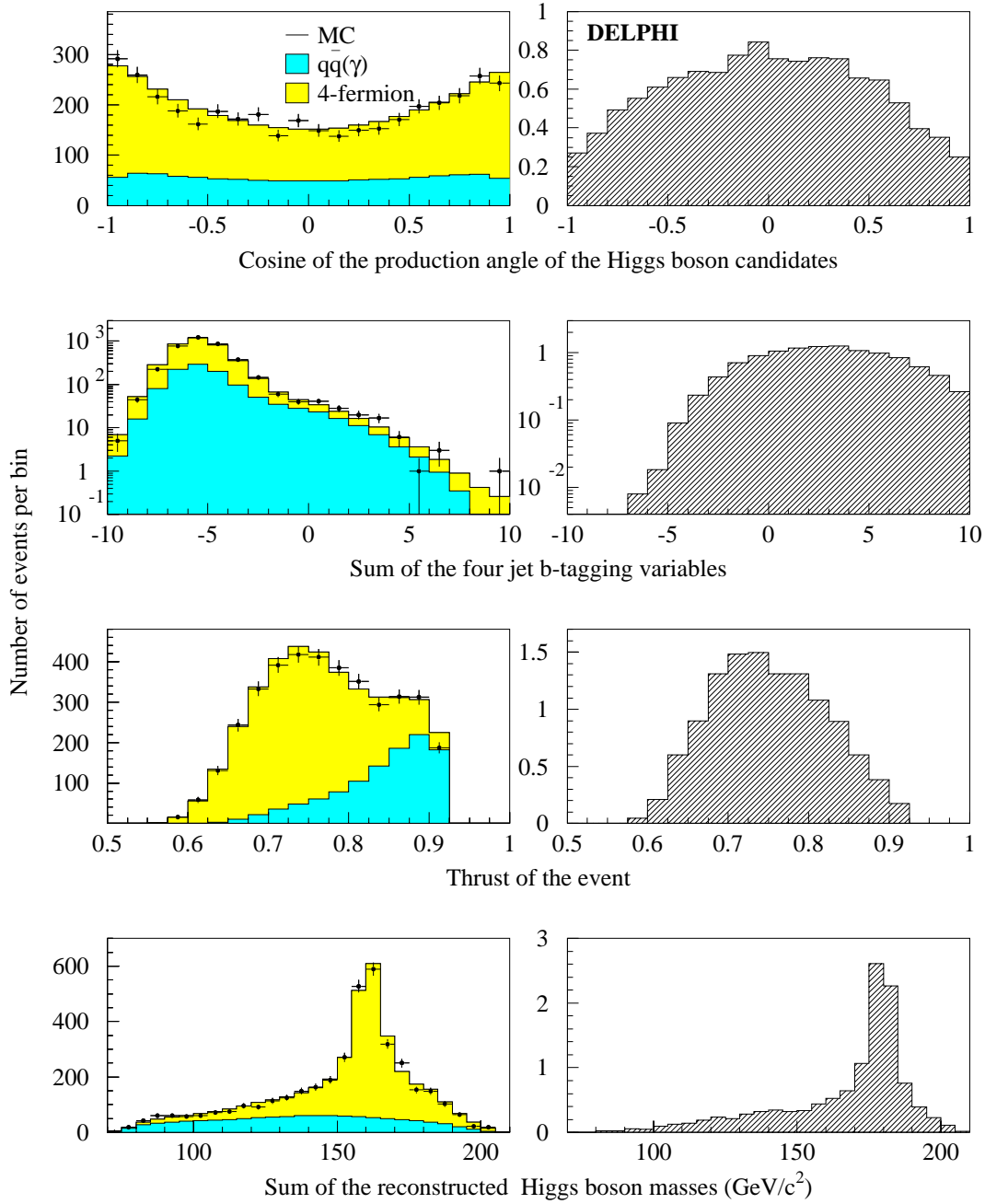
Figure 18: hA hadronic channel: distributions of four analysis variables, as described in the text, at preselection level. Data from the years 1999 to 2000 (dots) are compared with SM background process expectations (left-hand side histograms). The expected distributions for a m_A = m_h = 90 \text{ GeV}/c^2 signal are shown in the right-hand side plots.
