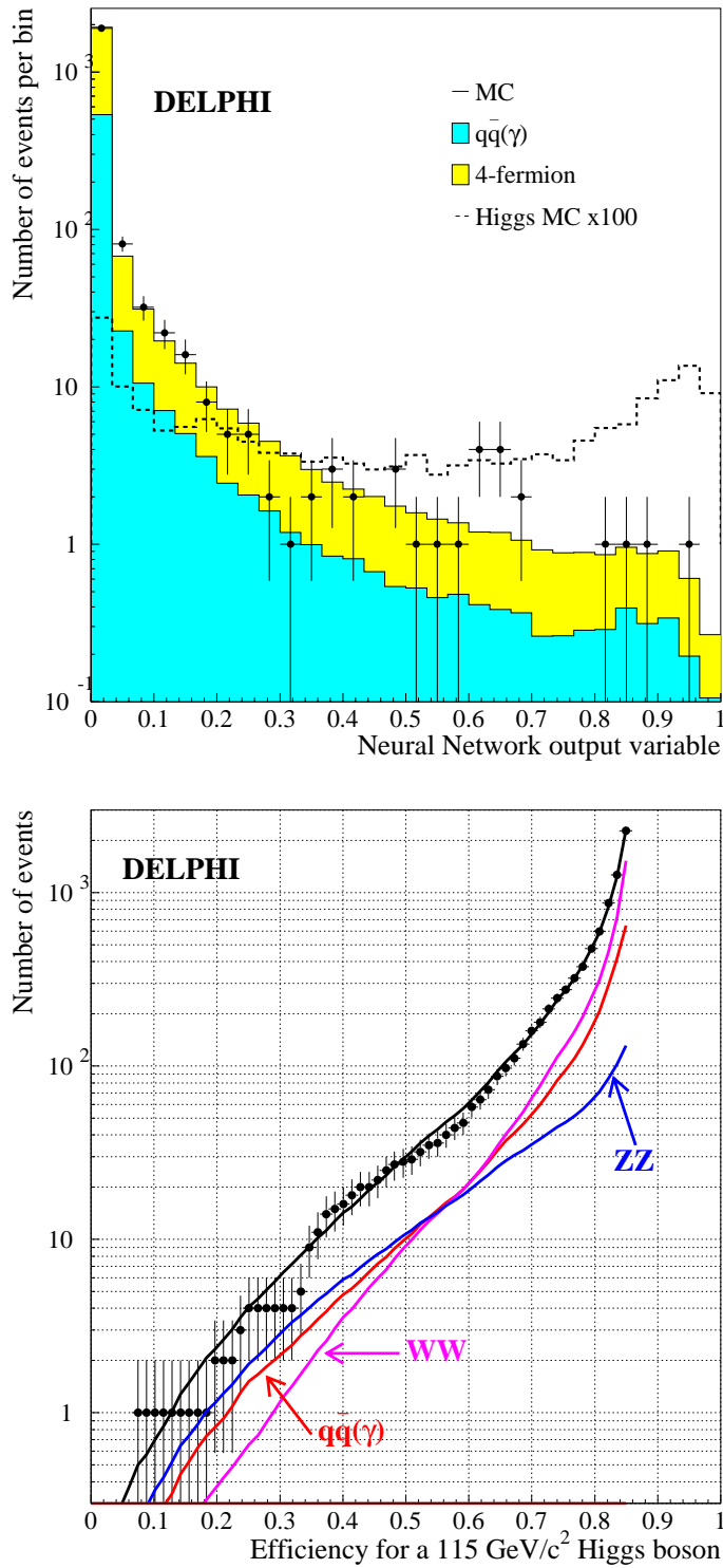
Figure 17: Hq\bar{q} channel: Top: the distribution of the neutral network variable used to select Higgs candidates in the 2000 data. The signal expectation is shown for a 115 \text{ GeV}/c^2 Higgs, normalised to 100 times the expected rate. The dots represent the data. Bottom: curve of the expected SM background rate in the 2000 data as a function of the efficiency for a 115 \text{ GeV}/c^2 Higgs signal when varying the cut on the neural network variable. The different background contributions are shown separately. The dots represent the data.
