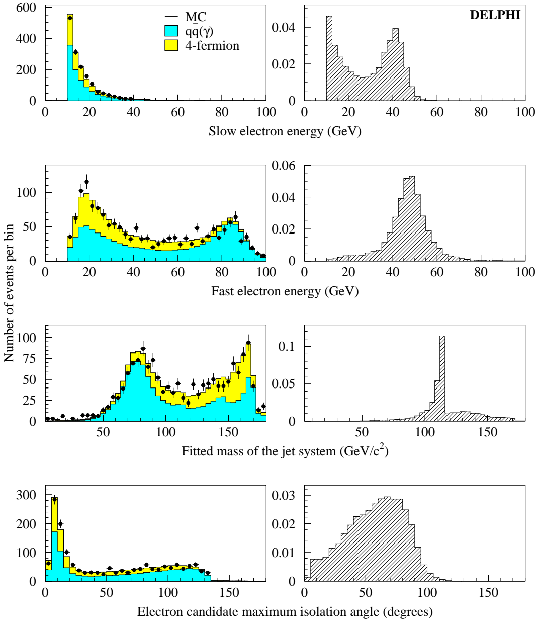
Figure 6: \text{He}^+e^- channel: distributions of four analysis variables, as described in the text, at preselection level. Data from the year 2000 (dots) are compared with SM background process expectations (left-hand side histograms). The expected distributions for a 115 \text{ GeV}/c^2 signal are shown in the right-hand side plots.
