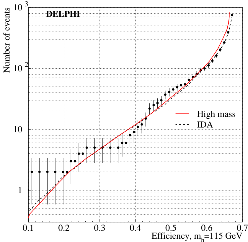
Figure 15: H\nu\bar{\nu} channel, IDA analysis: the observed rate and that expected from the SM background processes as a function of the efficiency for a 115 \text{ GeV}/c^2 Higgs signal when varying the cut on the IDA variable. The solid curve, from the high mass analysis, is included so that the very similar performance of the two analyses can be seen. The dots represent the data.
