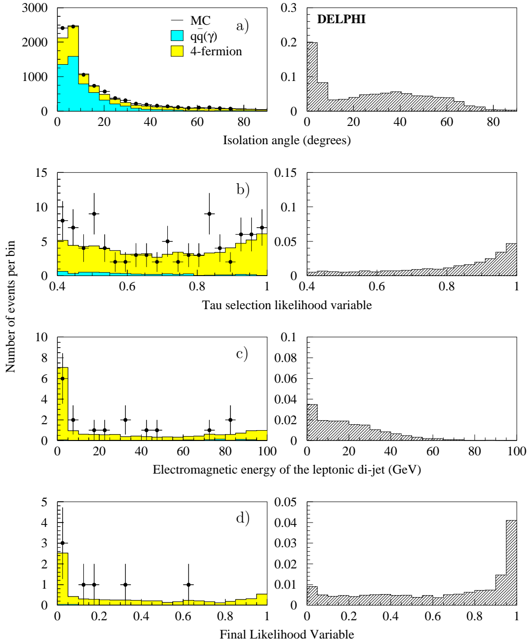
Figure 8: \tau^+\tau^-q\bar{q} channel: distributions of four analysis variables at different levels of the selection, as described in the text. Data from the year 2000 (dots) are compared with SM background process expectations (left-hand side histograms). The expected distributions for a 115 \text{ GeV}/c^2 Higgs signal in the (H \rightarrow \tau^+\tau^-)(Z \rightarrow q\bar{q}) channel are shown in the right-hand side plots.
