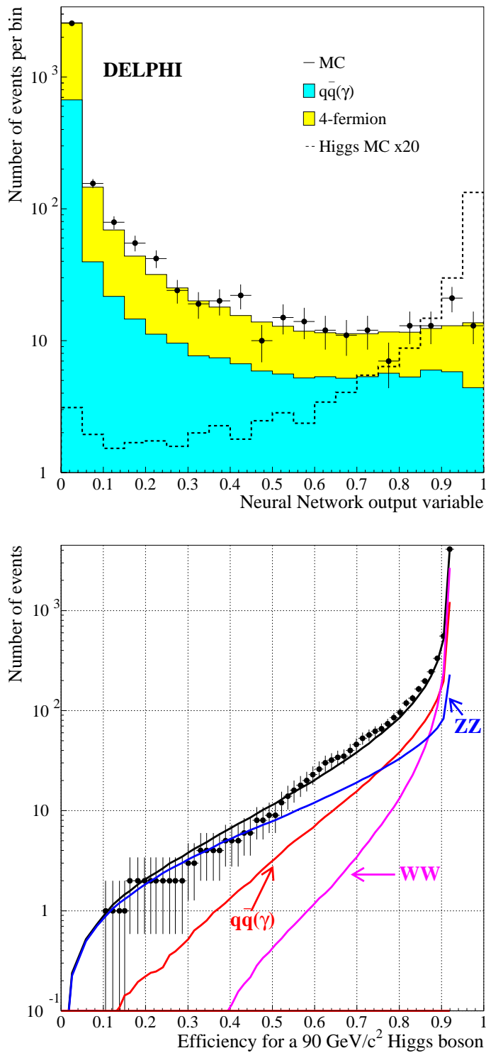
Figure 19: hA hadronic channel: Top: distributions of the ANN variable for the expected SM background processes (full histograms), the data from the years 1999 and 2000 (dots) and the expected m_A = m_h = 90 \text{ GeV}/c^2 Higgs signal (dashed histogram, normalised to 20 times the expected rate). Bottom: curve of the expected SM background rate for all data from 1999 and 2000 as a function of the efficiency for the same signal when varying the cut on the ANN variable. The different background contributions are shown separately. The dots show the data.
