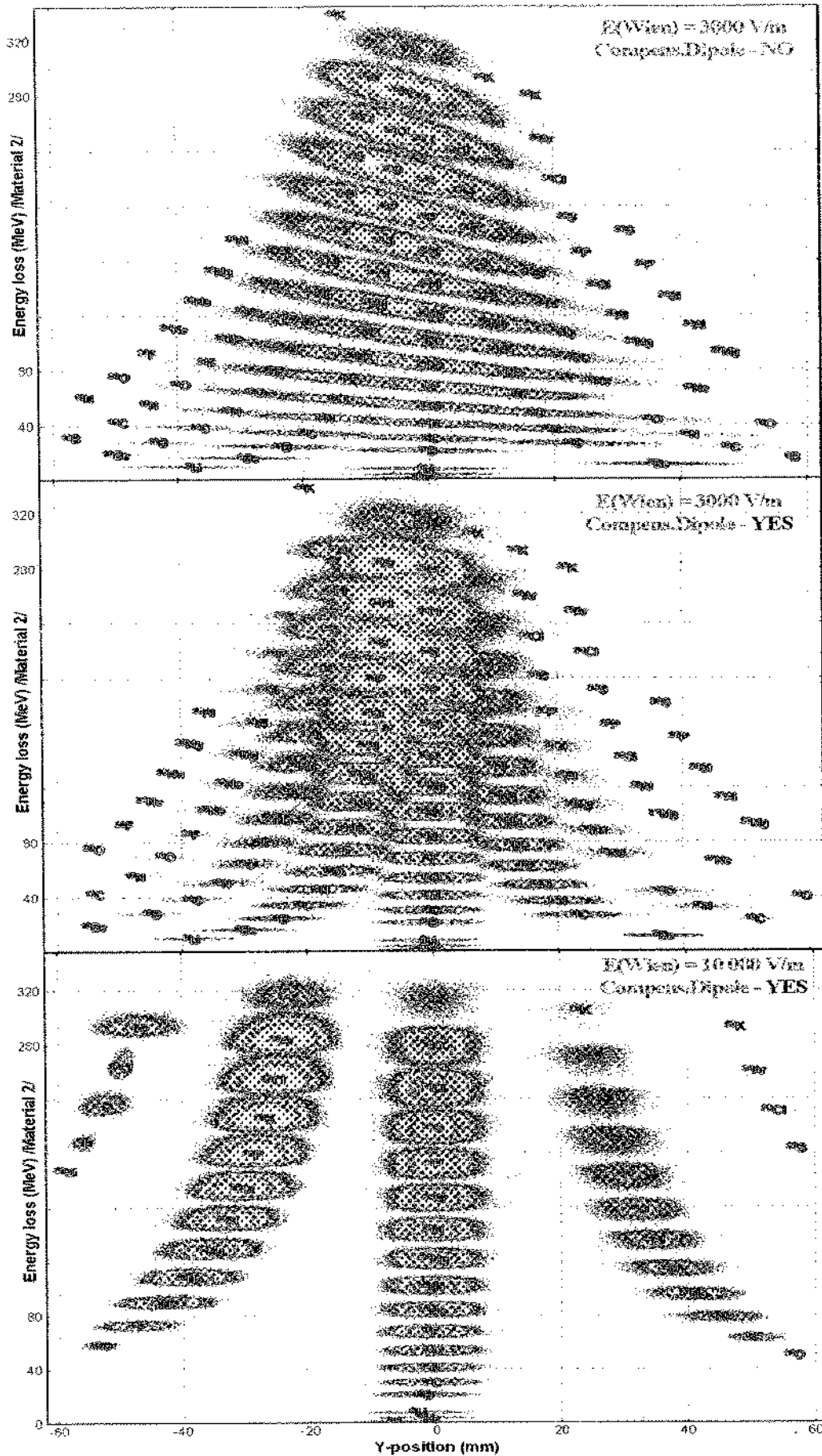
Fig.15. dE - Y simulation spectra for the reaction ^{40}\text{Ar} + \text{Be}(500 \mu\text{m}) with ^{32}\text{S} as the setting fragment. The LISE spectrometer ( \Delta p/p=4.6\% ), Wien velocity filter and the compensating dipole were used in the calculations. LISE velocity filter selects fragments in the vertical plane. Energy loss calculations were done through a 300 \mu\text{m} silicon detector located behind the compensating dipole.
