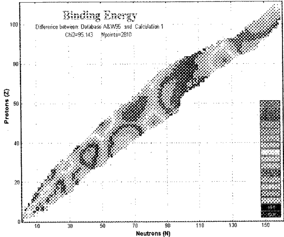
Fig.30. Differences between binding energies of the inbuilt database and LDM1 parameterization.
