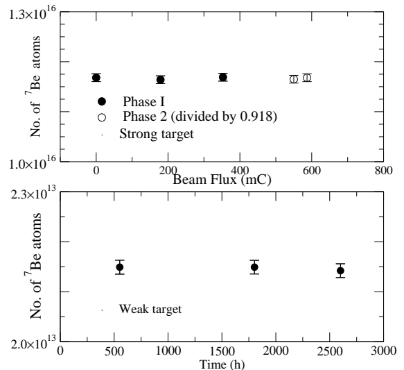
FIG. 11: Top: The {}^7\text{Be} target content, determined by measuring the activity in a Ge detector, as a function of the accumulated charge on target and corrected for the decay of {}^7\text{Be} . The open circles are scaled by a factor of 0.918 (see text). Bottom: The number of {}^7\text{Be} atoms corrected for decay in the weak target as function of time.
