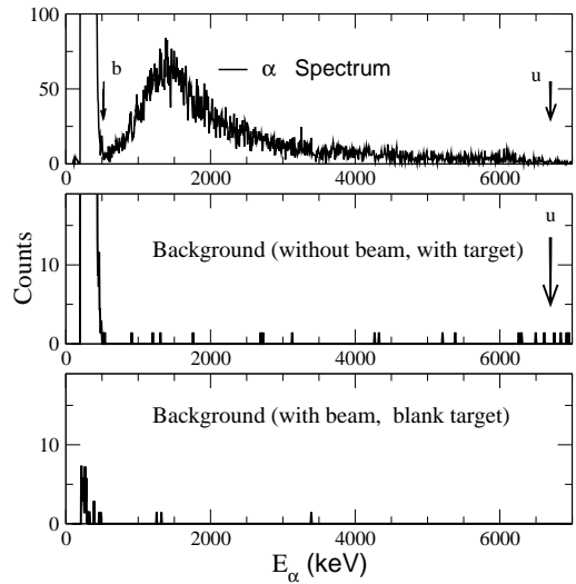
FIG. 6: Top: An \alpha spectrum obtained at E_{lab} = 991 keV in the geometry (1). This spectrum was collected over a time of \approx 40 hours. Middle: A background spectrum collected without beam and the target in front of the detector for a time of \approx 33 hours. The noise cut-off is at E_\alpha \approx 525 keV. Bottom: Background spectrum collected for a time of \approx 5 hours with the {}^7\text{Be} target replaced by a copper blank.
