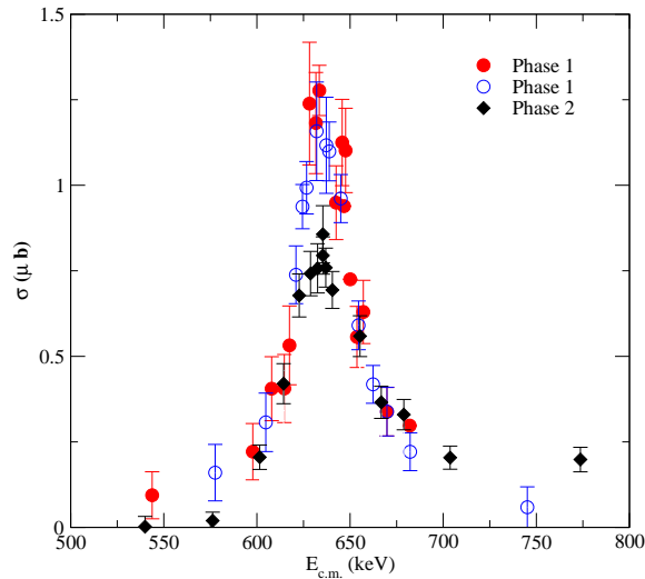
FIG. 10: Measurements around the 633 keV resonance in phase 1 and phase 2.
