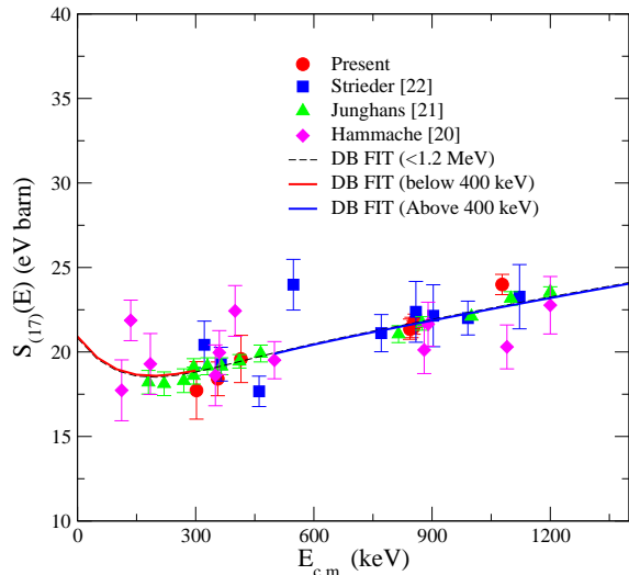
FIG. 17: Non resonant part of the S_{17}(E) from recent direct capture measurements. Each set of S_{17}(E) values was fitted independently to the DB parameterization and the individual scaling factors were then renormalized to a reference value corresponding to S_{17}(0) = 21.2 eV barn. The overall consistency of the data upto E_{c.m.} = 1.2 MeV as well as the agreement with the DB parameterization is apparent.
