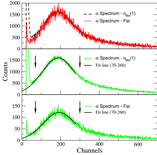
FIG. 8: Top: The \alpha spectrum from the {}^7\text{Li}(d,p){}^8\text{Li} reaction for the near geometry (1) and the corresponding far geometry scaled to coincide at the peak. Middle and Bottom: The individual \alpha spectra and the respective Gaussian fits in the region between the markers.
