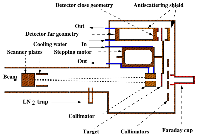
FIG. 1: A schematic view of the experimental setup.
