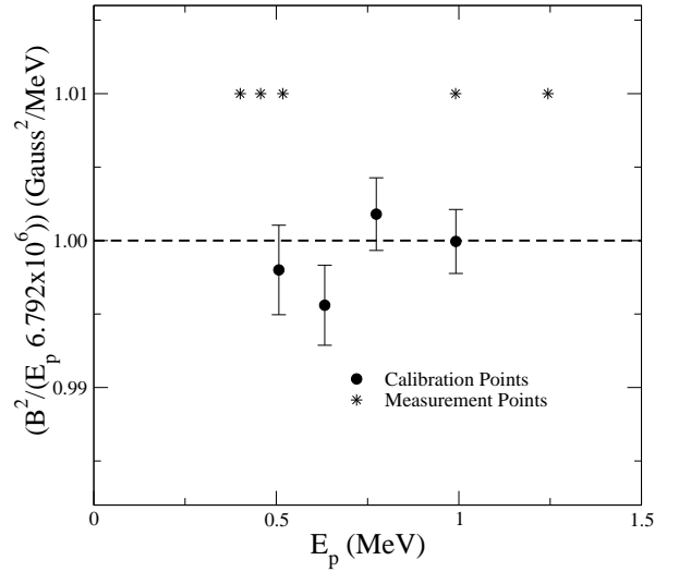
FIG. 4: Energy calibration of the Van de Graaff accelerator. The circles represent the calibration points and the ‘*’ represent the energies at which {}^7\text{Be}(p,\gamma){}^8\text{B} measurements were carried out. The constant (6.79 \pm 0.02) \times 10^6 Gauss ^2 /MeV used to scale the Y-axis is obtained from the fit as described in the text (section II B).
