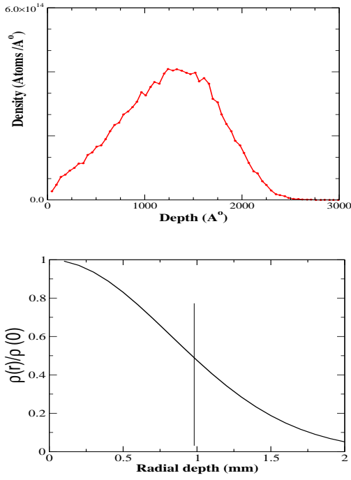
FIG. 3: Top: The simulated depth distribution of 60 keV {}^7\text{Be} in copper. Bottom: The areal density distribution of {}^7\text{Be} beam used for implantation at ISOLDE, this is also the {}^7\text{Be} density distribution in the target. The vertical line indicates the edge of the implanted target. (see II A for details).
