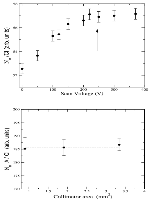
FIG. 5: Top: \alpha yield from the ^7\text{Li}(d,p)^8\text{Li} reaction at E_d = 770 \text{ keV} , normalized to the integrated beam current as a function of the scan voltage. The scan voltage used in the experiment, scaled to the corresponding beam energy, is indicated by the marker. Bottom: \alpha yield from the ^7\text{Li}(d,p)^8\text{Li} reaction for various collimators normalized to the integrated beam current and multiplied by the area of the collimator.
