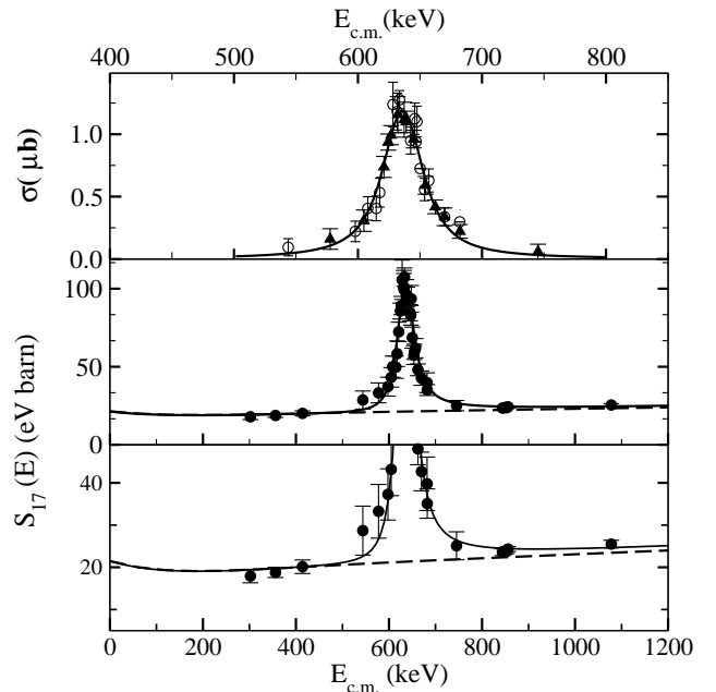
FIG. 16: Top: The resonance at 633 keV. The points are the measured cross sections after subtraction of the non-resonant part. The energy axis is expanded in comparison to the middle and lower panel. The two symbols represent two separate measurements. The continuous curve represents the convolution of a Breit-Wigner resonance with the simulated ^7\text{Be} distribution in Cu. Middle: The points are the measured S_{17}(E) . The continuous line is the scaled function of Descouvemont and Baye [DB] [34] plus a Breit-Wigner resonance with an energy dependent width. The dashed line is the scaled DB model. Bottom:- An expanded view of the middle figure.
