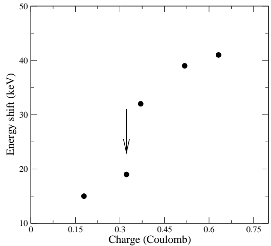
FIG. 13: The energy shift of the centroid of the 633 keV resonance due to carbon buildup on the target, as a function of the integrated charge. The marker indicates the ‘thermal episode’ (see text).
