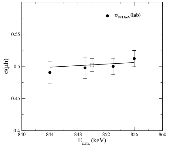
FIG. 15: The cross section for {}^7\text{Be}(p,\gamma){}^8\text{B} measured at different geometries at E_{\text{lab}}=991 keV. The gradual energy shift is due to the carbon build up on the target. The solid line is from Eqn.10 The open circle represents the average cross section at E_{\text{c.m.}}=850 keV
