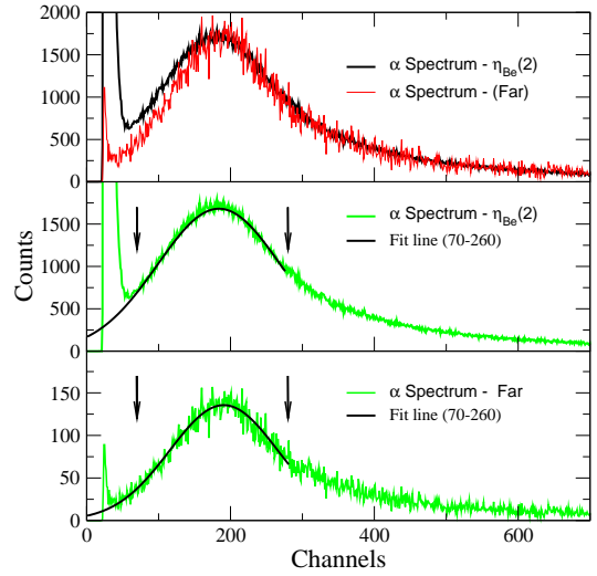
FIG. 9: Top: The \alpha spectrum from the {}^7\text{Li}(d,p){}^8\text{Li} reaction at near geometry (2) and the corresponding far geometry scaled to coincide at the peak. Middle and Bottom: The individual \alpha spectra and the respective Gaussian fits in the region between the markers.
