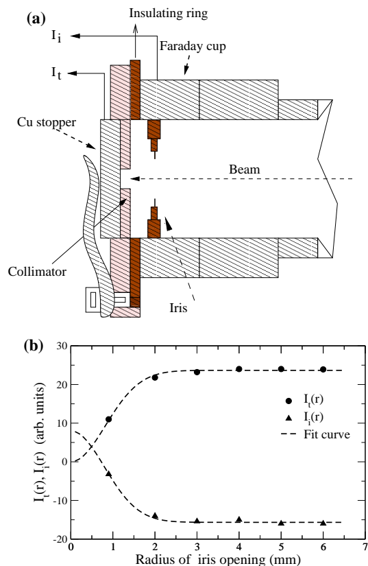
FIG. 2: (a): A schematic view of the implantation chamber. Note the collimator of 2 mm diameter in the beam path that defines the dimensions of the {}^7\text{Be} spot. (b): The measured beam profiles as function of the iris opening.
