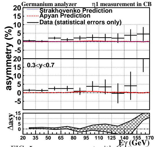
FIG. 5: \eta_1 measurement with Ge target
