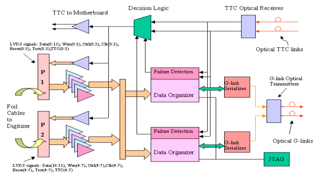
Figure 3: Interface Functional System Structure.
