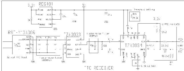
Figure 4: Schematic of TTC receiver.
