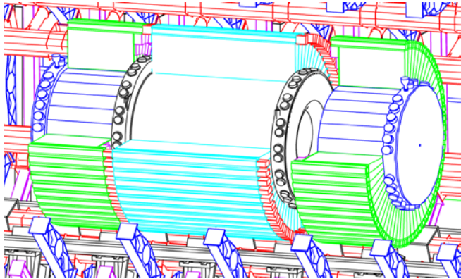
Figure 1: The Tile Calorimeter
