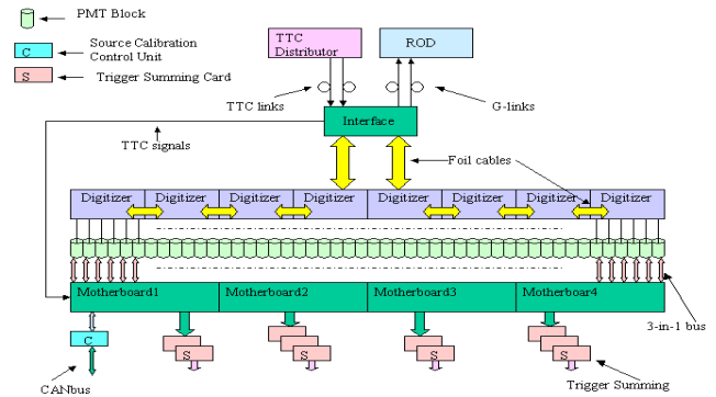
Figure 2: TileCal Readout Electronics Diagram
