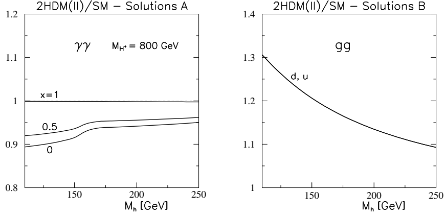
Figure 1: Ratios of the Higgs boson decay widths in the SM-like 2HDM (II) and the SM as functions of M_h . Left panel: h \rightarrow \gamma\gamma decay widths, solutions A, for M_{H^\pm} = 800 GeV and \mu/\sqrt{2} = xM_{H^\pm} . Right panel: h \rightarrow gg , solutions B.
