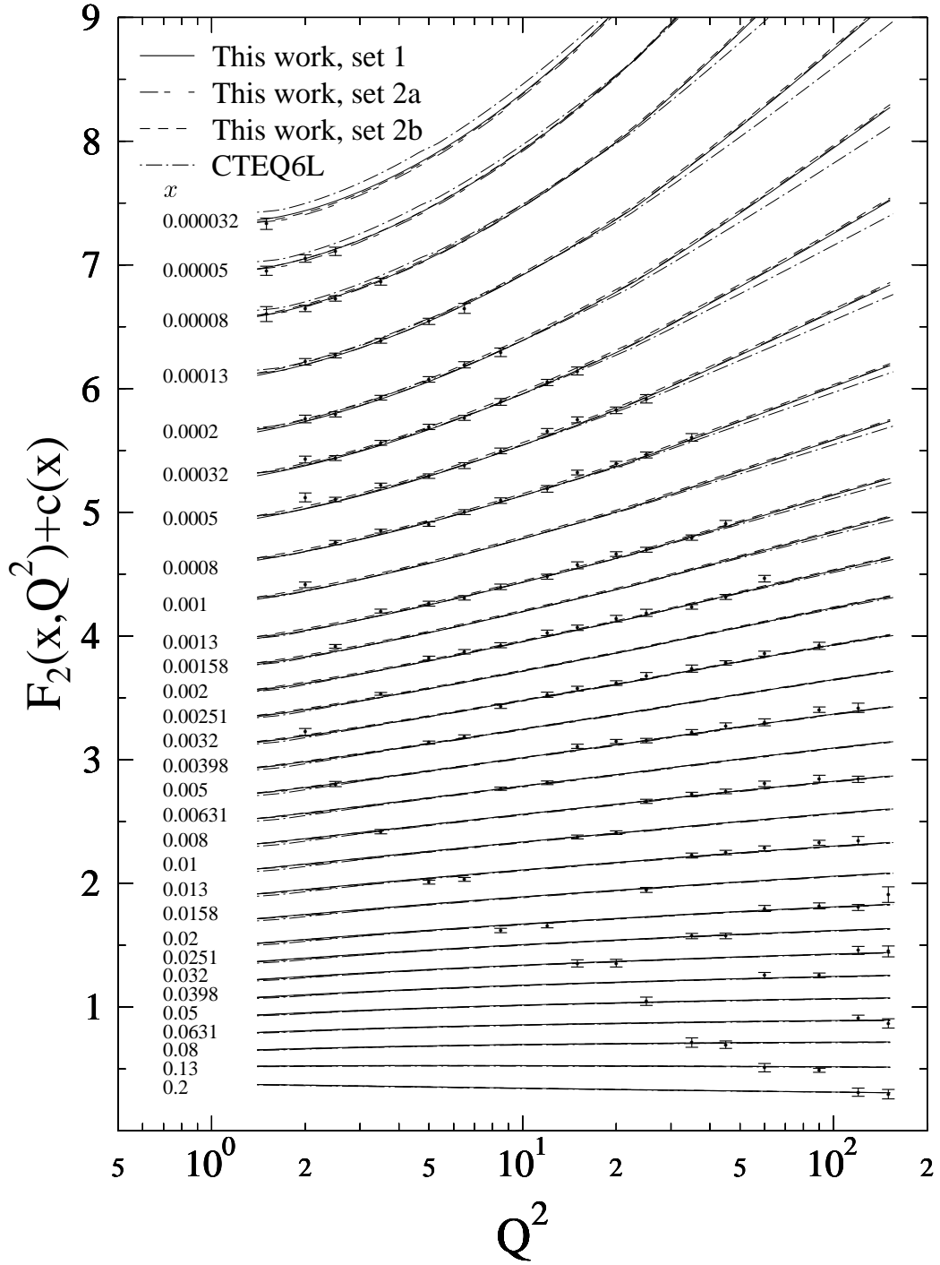
Figure 3: As Fig. 1 but for LO DGLAP result from CTEQ6L (dotted-dashed) and for the DGLAP+GLRMQ results with our set 1 (solid), set 2a (double dashed) and set 2b (short dashed).
