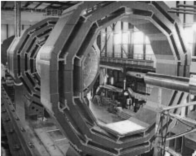
Fig. 2. Perspective view of the barrel yoke rings already assembled in the surface hall, showing pockets in which muon stations will be inserted. The outer vacuum tank, supported from the central barrel ring and destined to house the superconducting coil, also is visible.
