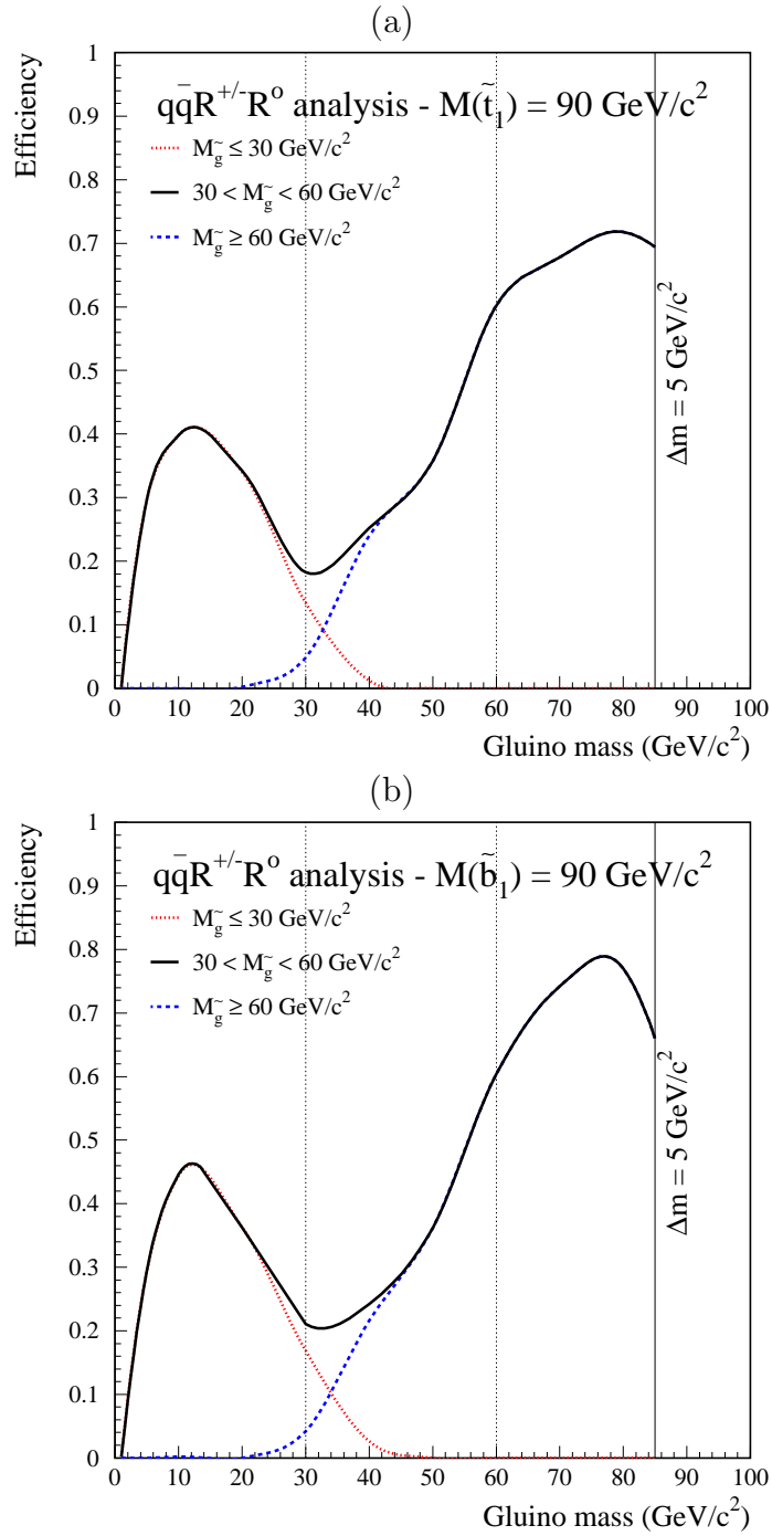
Figure 12: Signal detection efficiencies at \sqrt{s} = 200 \text{ GeV} for the stop (a) and sbottom (b) \bar{q}qR^{\pm}R^0 analysis as a function of the gluino mass ( m_{\tilde{q}_1} = 90 \text{ GeV}/c^2 ). \Delta M is the mass difference between the squark and the gluino. Vertical lines show the limits of the mass analysis window. The last one ends at \Delta M = 5 \text{ GeV}/c^2 which corresponds the last simulated signal points.
