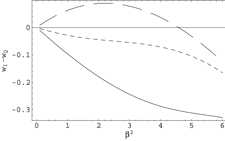
Figure 1: Plot of w_I - w_Q as a function of \beta^2 for n = 2 . The long dashed curve corresponds to t/\tau = 1 , the short dashed curve corresponds to t/\tau = 5 , and the solid curve corresponds to t/\tau = 10 .
