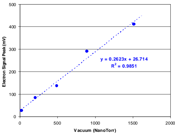
Figure 5. Prompt electron signal amplitude plotted as a function of local vacuum pressure. All other beam parameters were held fixed.
