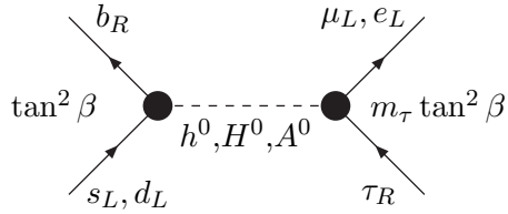
Figure 1: Dominant Higgs penguin diagrams contributing to (a) B_{s,d}^0 \rightarrow \mu\mu and (b) \tau \rightarrow \mu\mu\mu decays at large \tan\beta .
