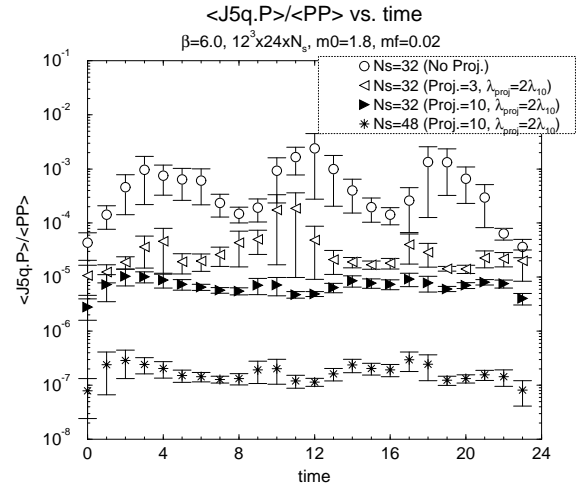
Figure 1. \frac{\langle J_{5q} P \rangle}{\langle P P \rangle} without and with projection for N_s = 32 and with projection for N_s = 48 . The fitting range for m_{\text{res}} is 4 \leq t \leq 20 .
