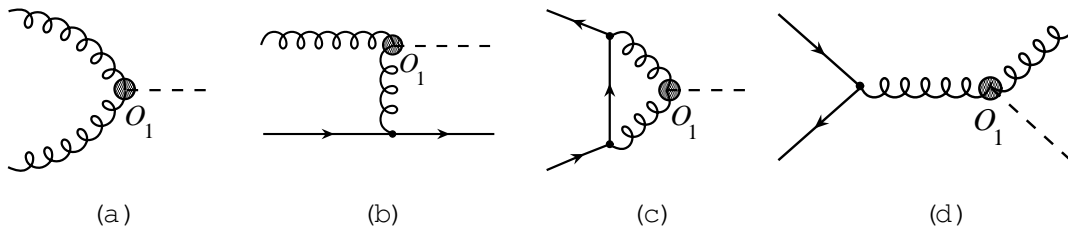
Figure 1: Sample diagrams for h\mathcal{O}_1^B . Higher orders are obtained by dressing these diagrams with additional quarks and gluons, both virtual and real.
