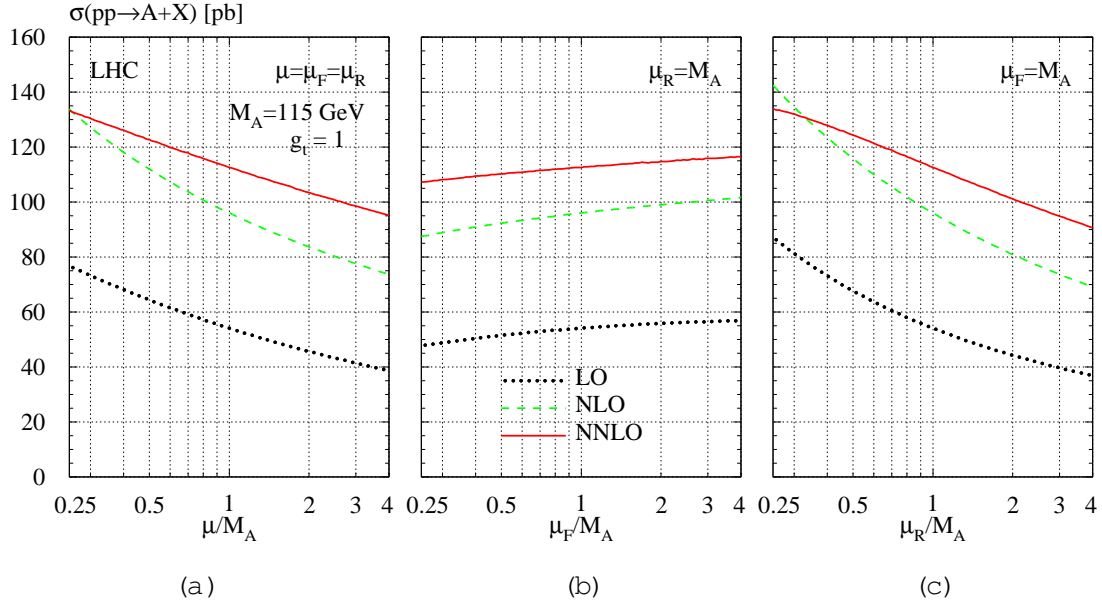
Figure 5: Scale dependence of the cross section for an M_A = 115 GeV pseudo-scalar Higgs boson at the LHC ( \sqrt{s} = 14 TeV) (a) varying \mu_F = \mu_R , (b) varying \mu_F, \mu_R = M_A and (c) varying \mu_R, \mu_F = M_A .
