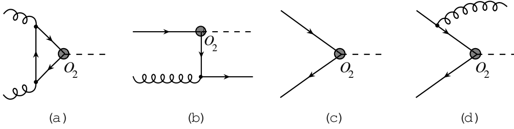
Figure 2: Sample diagrams for h\mathcal{O}_2^B i as required up to NNLO.
