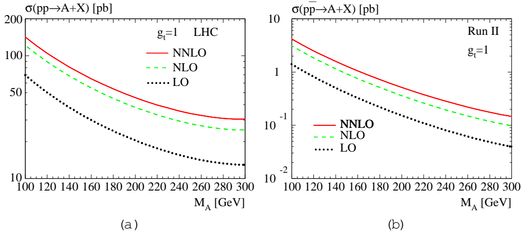
Figure 3: Total cross section for inclusive production of pseudo-scalar Higgs bosons ( A ) at (a) the LHC ( \sqrt{s} = 14 \text{ TeV} ) and (b) Tevatron Run II ( \sqrt{s} = 2 \text{ TeV} ). The coupling constant for the coupling of A to top quarks is such that g_t = 1 . The cross section for other values of g_t (e.g., g_t = \cot \beta in the MSSM) can be obtained by scaling the curves with |g_t|^2 .
