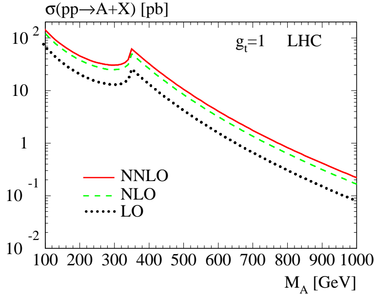
Figure 4: Total cross section for inclusive production of pseudo-scalar Higgs bosons ( A ) at the LHC ( \sqrt{s} = 14 \text{ TeV} ), as in Fig.3 for a larger mass range. The cusp is an effect of the top-quark threshold.
