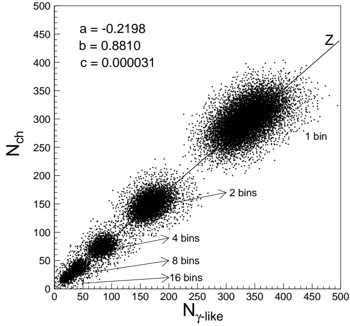
FIG. 4: The event-by-event correlation between N_{\text{ch}} and N_{\gamma\text{-like}} for centrality bin=1. Overlaid on the plot is the common correlation axis (Z-axis) obtained for the full distribution by fitting the N_{\gamma\text{-like}} and N_{\text{ch}} correlation with a second order polynomial. The values in the upper left are the coefficients of the polynomial of the form N_{\text{ch}} = a + bN_{\gamma\text{-like}} + cN_{\gamma\text{-like}}^2 . For the other three centrality classes, the plots are qualitatively similar.
