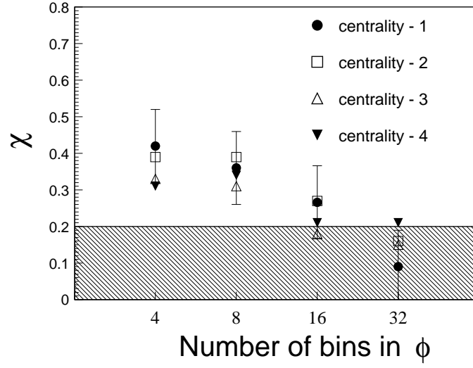
FIG. 10: The fluctuation strength parameter for the four centrality classes. Centrality-1 corresponds to the 5% most central, centrality-2 corresponds to 5 – 10%, centrality-3 corresponds to 15 – 30% and centrality-4 corresponds to 45 – 55% of the minimum bias cross section as determined by selection on the measured transverse energy distribution. The error bars are shown only on the centrality-1 selection for clarity of presentation. The errors are similar for the other centralities. The shaded portion represents the limit above which a signal is detectable (see text for details).
