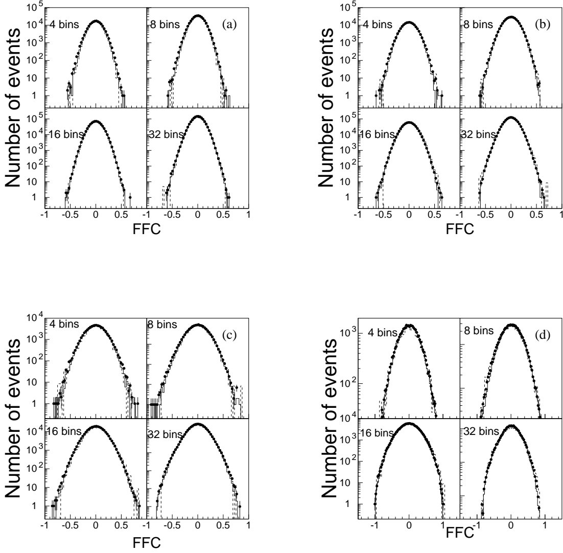
FIG. 8: The FFC distributions for data (solid circles), mixed events (solid histogram), and simulation (dashed histogram) for the four centrality bins (a) centrality-1 (0–5%), (b) centrality-2 (5–10%), (c) centrality-3 (15–30%), (d) centrality-4 (45–55%).
