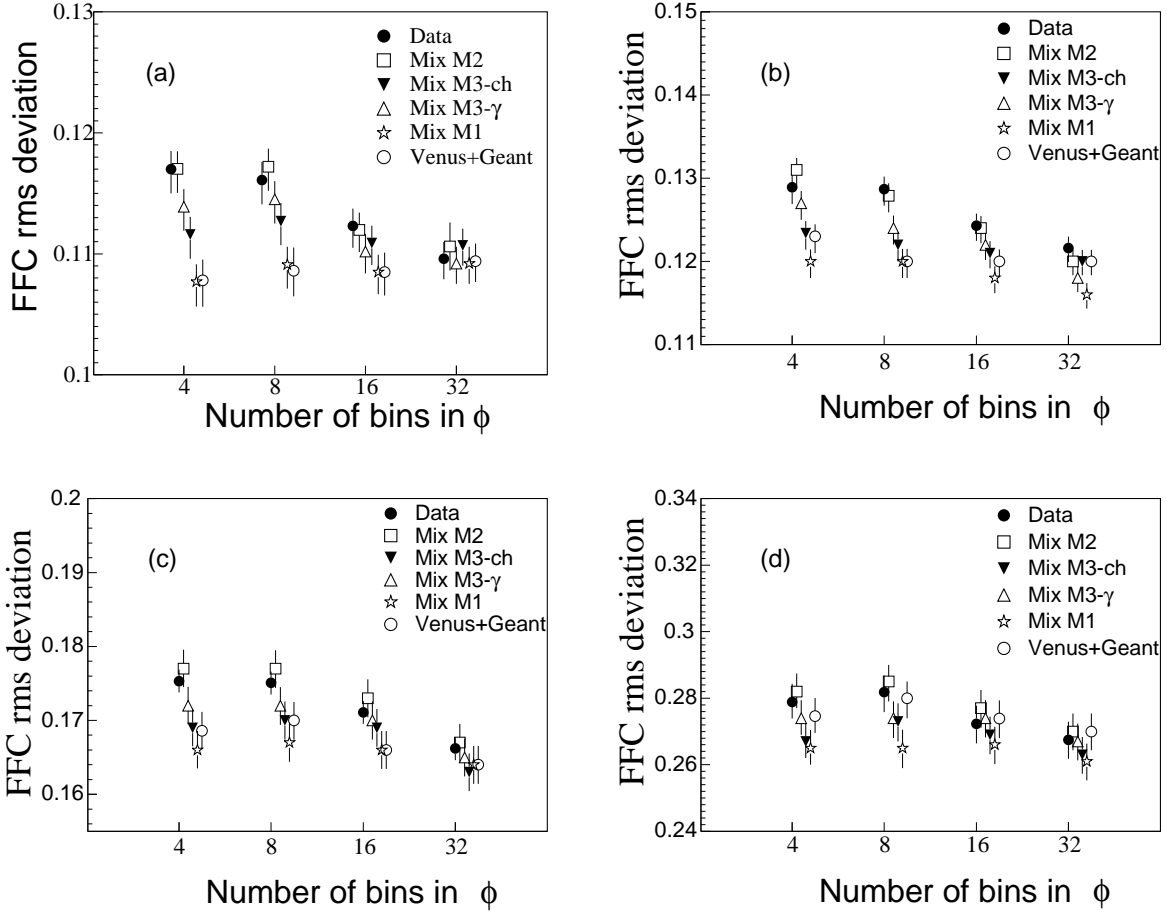
FIG. 9: The RMS deviations of the FFC distributions for data, various mixed events, and simulation for the four centrality bins (a) centrality-1 (0 – 5%), (b) centrality-2 (5 – 10%), (c) centrality-3 (15 – 30%), (d) centrality-4 (45 – 55%).
