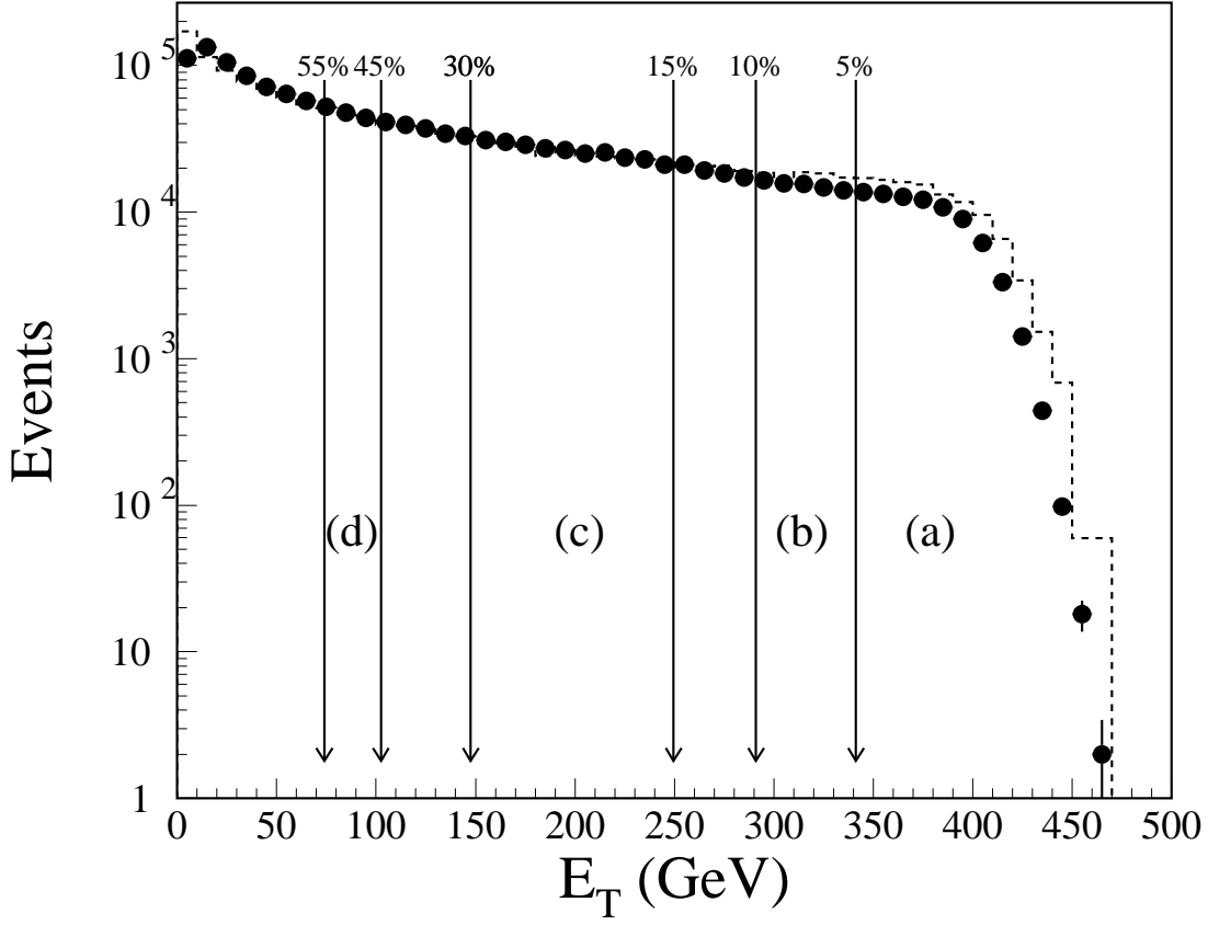
FIG. 1: The total E_T distribution (solid dots) measured in 3.5 \leq \eta \leq 5.5 for Pb+Pb collision at 158 A GeV/c. The total E_T distribution as obtained from VENUS is also shown as dashed histogram. The E_T values corresponding to the different centrality bins used in the analysis are shown. (a) centrality-1 (0 – 5%), (b) centrality-2 (5 – 10%), (c) centrality-3 (15 – 30%), (d) centrality-4 (45 – 55%) of the minimum bias cross section as determined by selection on the measured transverse energy distribution.
