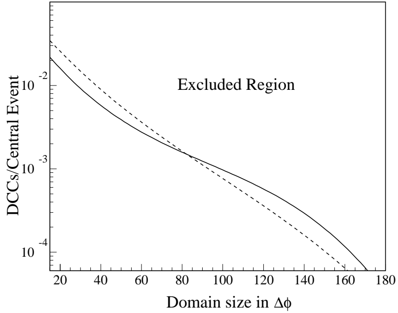
FIG. 11: The 90% confidence level upper limit on DCC production for central Pb+Pb collision at 158 A GeV/c, as a function of the DCC domain size in azimuthal angle within the context of a simple DCC model and the measured photon and charged particle multiplicities in the interval 2.9 < \eta < 3.75 . The solid line corresponds to data from the top 5% and dashed line to top 5 – 10% of the minimum bias cross section as determined by selection on the measured transverse energy distribution.
