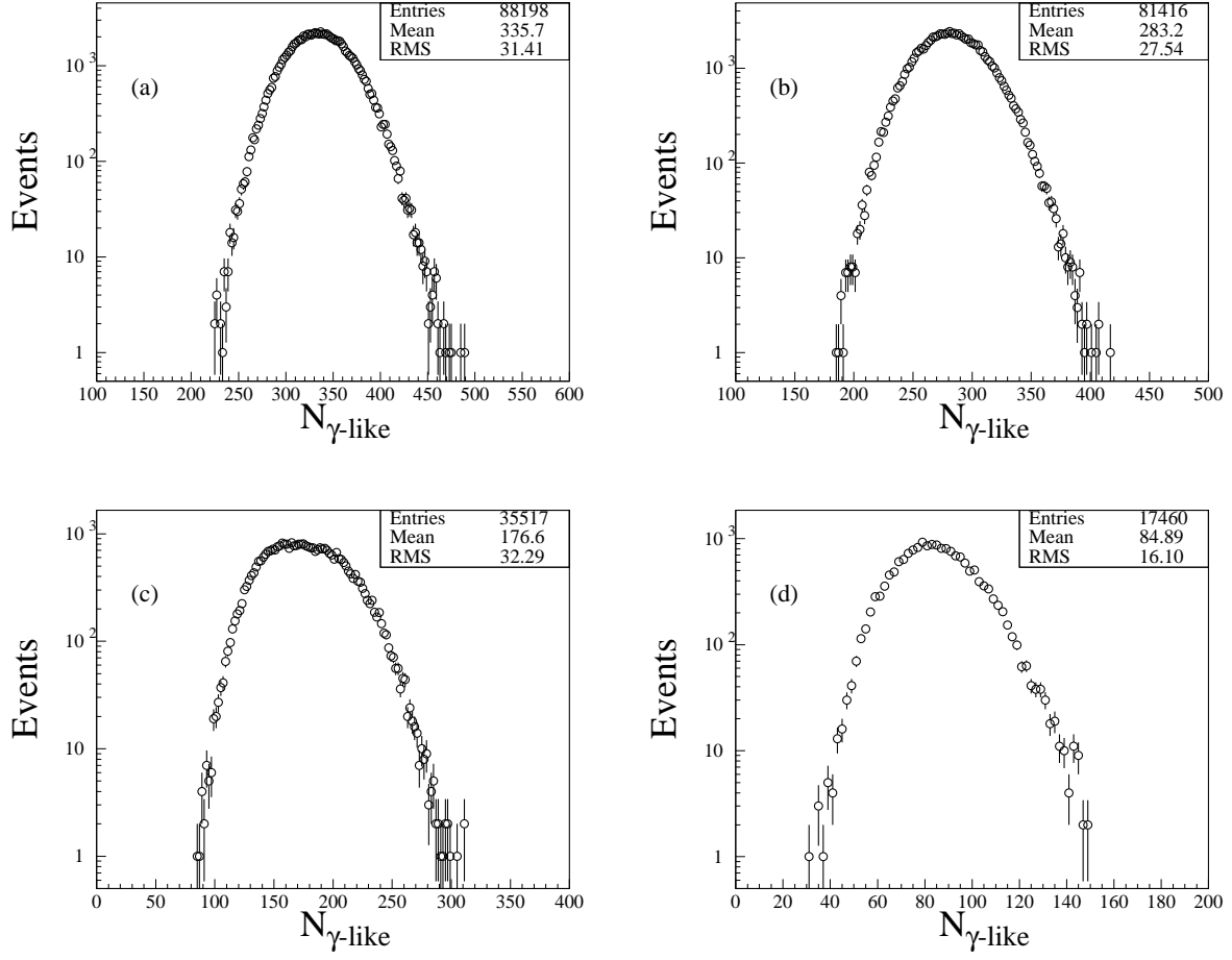
FIG. 2: The N_{\gamma\text{-like}} multiplicity distributions for the four centrality selections for Pb+Pb collision at 158 A GeV/c. (a) centrality-1 (0 – 5%), (b) centrality-2 (5 – 10%), (c) centrality-3 (15 – 30%), (d) centrality-4 (45 – 55%).
