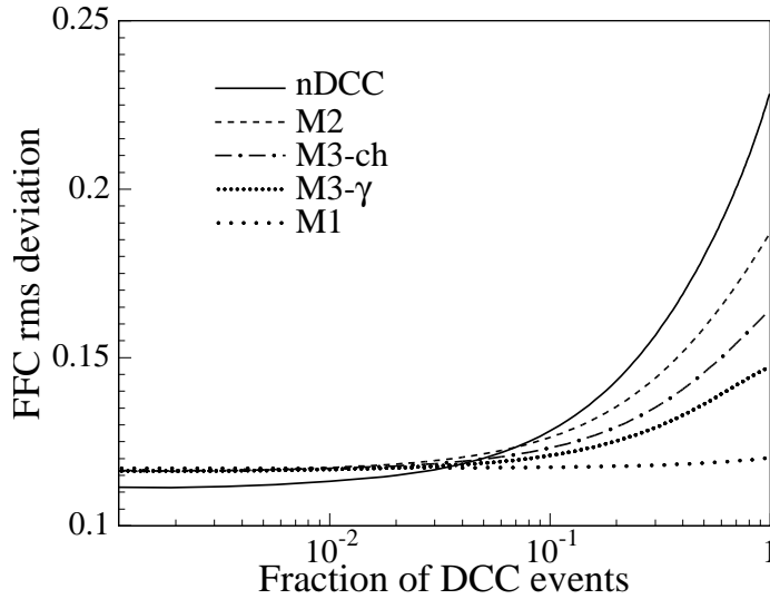
FIG. 5: The rms deviations of the FFC distributions for simulated VENUS events containing a variable fraction of localized DCC-like events with DCC extent \Delta\phi_{\text{DCC}} = 90^\circ , as a function of that fraction. Results are also shown for various mixed events constructed from those events.
