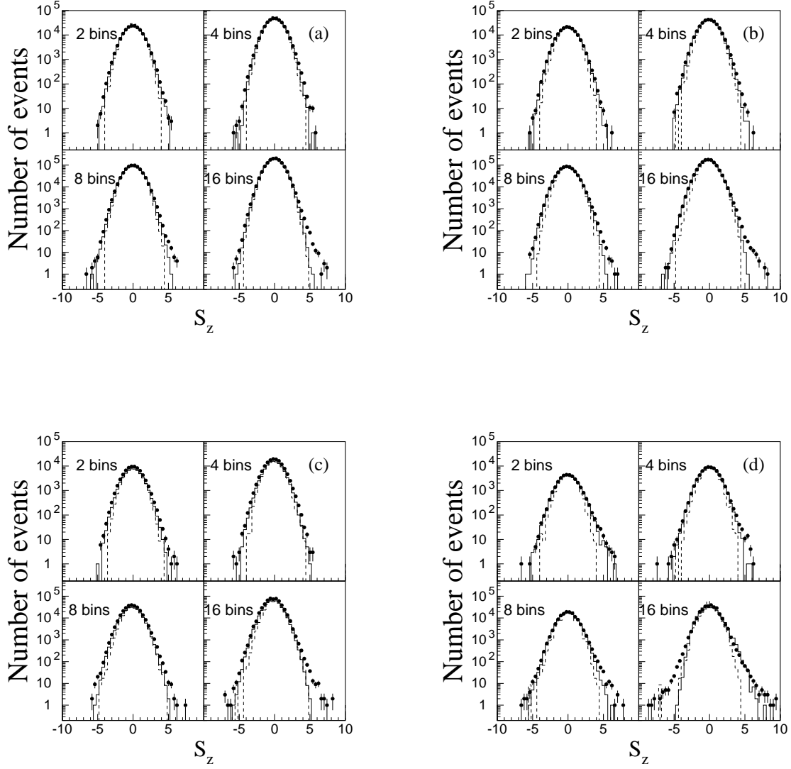
FIG. 6: The S_Z distributions for data (solid circles), mixed events (solid histogram), and simulated events (dashed histogram) for the four centrality bins (a) centrality-1 (0–5%), (b) centrality-2 (5–10%), (c) centrality-3 (15–30%), (d) centrality-4 (45–55%).
