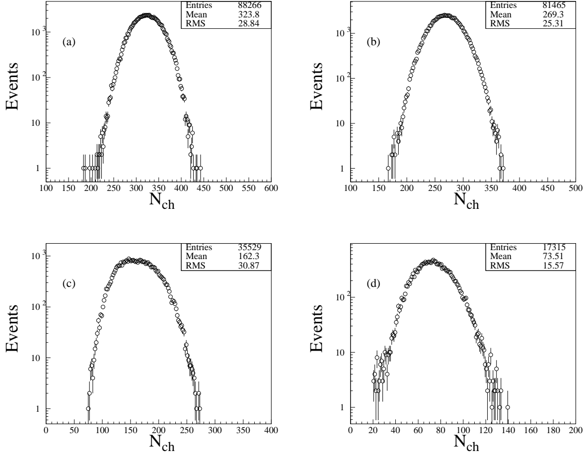
FIG. 3: The N_{\text{ch}} multiplicity distributions for the four centrality selections for Pb+Pb collision at 158 A GeV/c. (a) centrality-1 (0 – 5%), (b) centrality-2 (5 – 10%), (c) centrality-3 (15 – 30%), (d) centrality-4 (45 – 55%).
