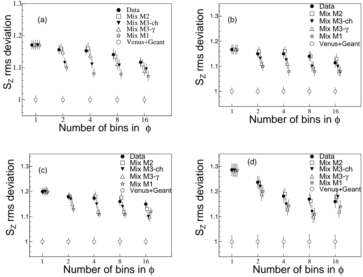
FIG. 7: The RMS deviations of the S_z distributions for data, various mixed events, and simulated events for the four centrality bins (a) centrality-1 (0 – 5%), (b) centrality-2 (5 – 10%), (c) centrality-3 (15 – 30%), (d) centrality-4 (45 – 55%).
