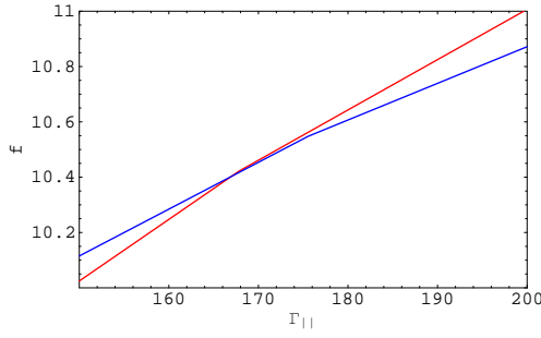
Figure 3: The free energies as functions of \Gamma_{\parallel} . Red - fluid and Blue - bcc.
