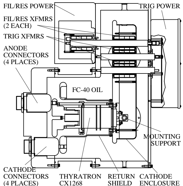
Figure 2, Thyatron and Final Enclosure
