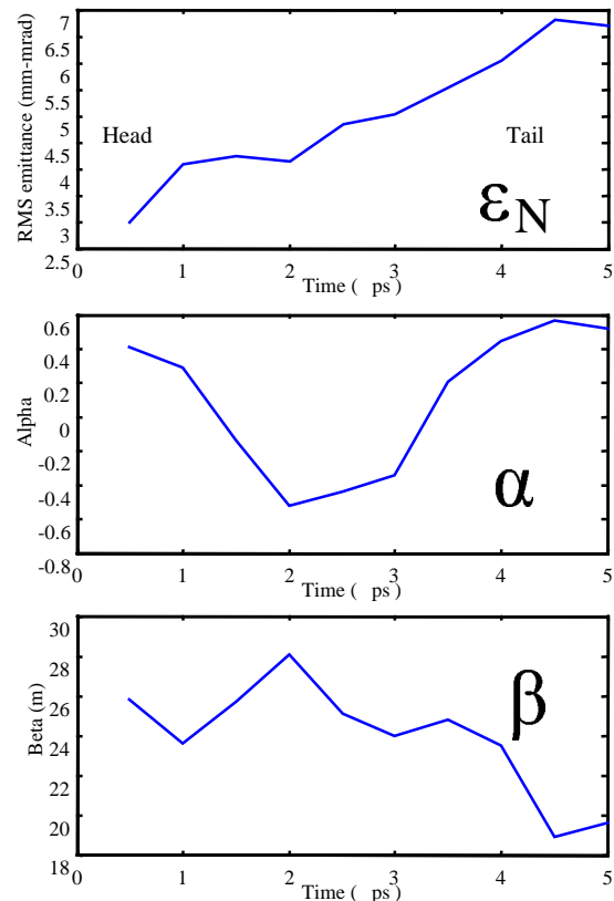
Figure 5: Vertical Twiss parameters as function of position in bunch. Slice width = 500 fs. Note substantial variation in slice emittance from head to tail, and symmetry of alpha.
