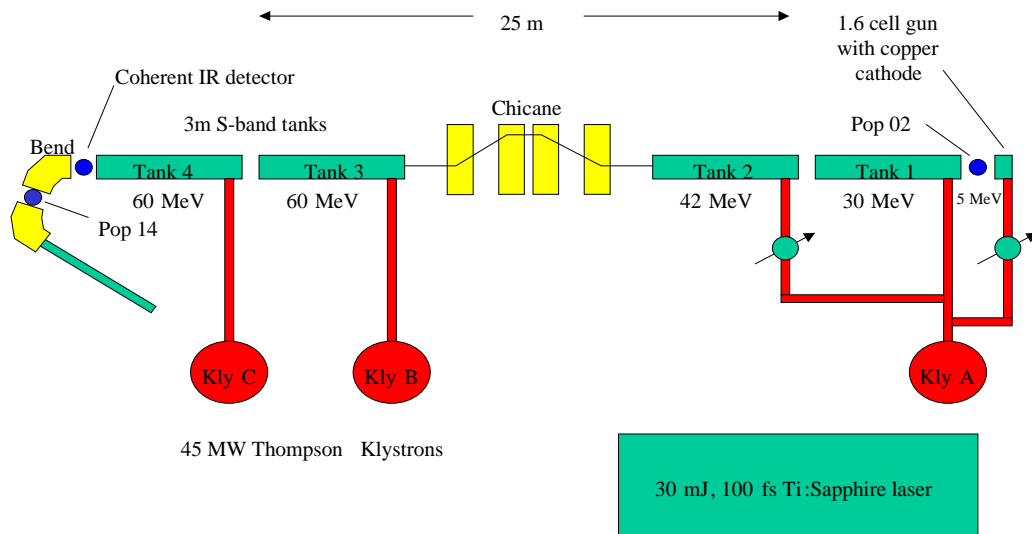
Figure 2: Layout of DUVFEL accelerator.
