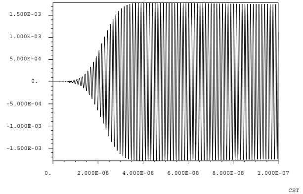
Figure 4: Magnetic field B_x(t) recorded as a function of time
