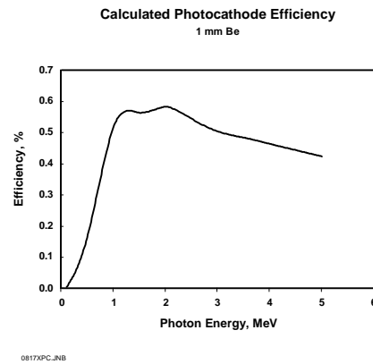
Figure 3: Pinhole framing camera photocathode response.
