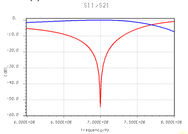
Figure 4: Transmission/Reflection Curve
