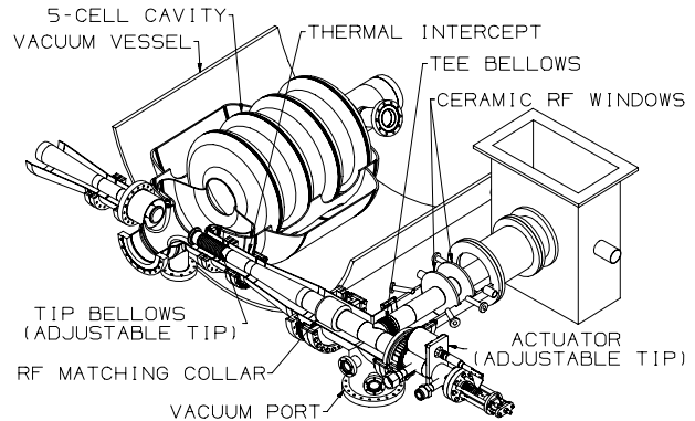
Figure 1: Power Coupler, Window, Cryomodule Assembly
