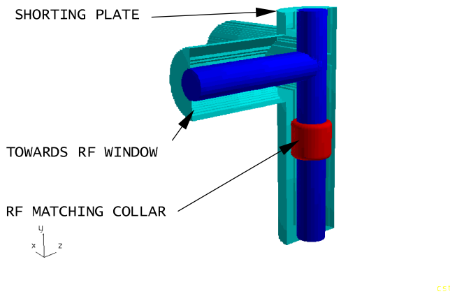
Figure 2: MAFIA Analytical Model
