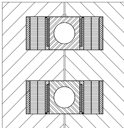
Figure 1 Cross section of the windings in the common coil magnet. The turns on the right form one half of the upper and lower dipoles, but are part of the same racetrack coil. Similarly, the turns on the left side form the other half of each dipole. The test windings are positioned inside the high current cable coils in a region of relatively uniform field.
