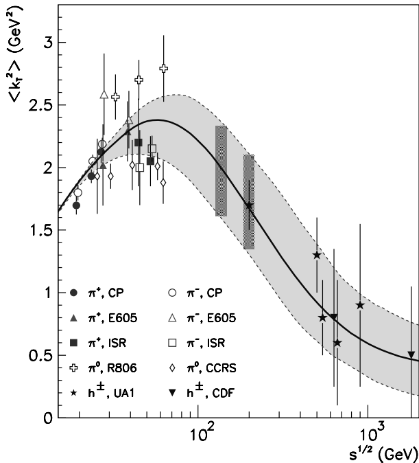
Fig. 1. The best fit values of \langle k_T^2 \rangle in pp \rightarrow \pi X [9,10] and p\bar{p} \rightarrow h^\pm X [11,12] reactions. Where large error bars would overlap at the same energy, one of the points has been shifted slightly for better visibility. The band is drawn to guide the eye.
