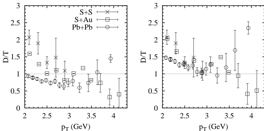
Fig. 2. Data/theory ratio at CERN SPS S+S (crosses), S+Au (boxes) and Pb+Pb (circles) for high p_T pion production reactions. Left: ratio without proton dissociation, right: ratio with proton dissociation after 4 collisions.
