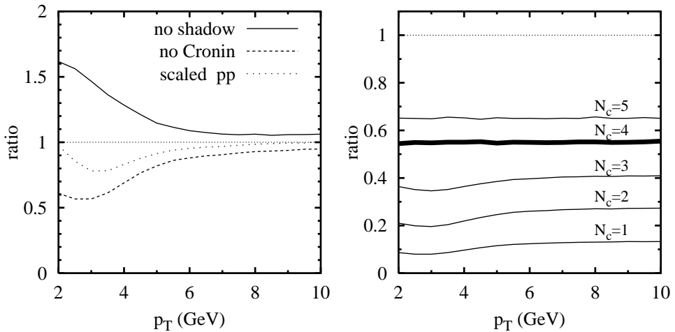
Fig. 3. Left: ratio of invariant cross section neglecting different terms as compared to the full pQCD calculation: neglecting shadowing (solid line), neglecting Cronin effect (dashed line), and neglecting both (dotted line). Right: ratio of invariant cross section with proton dissociation compared to the full pQCD calculation.
