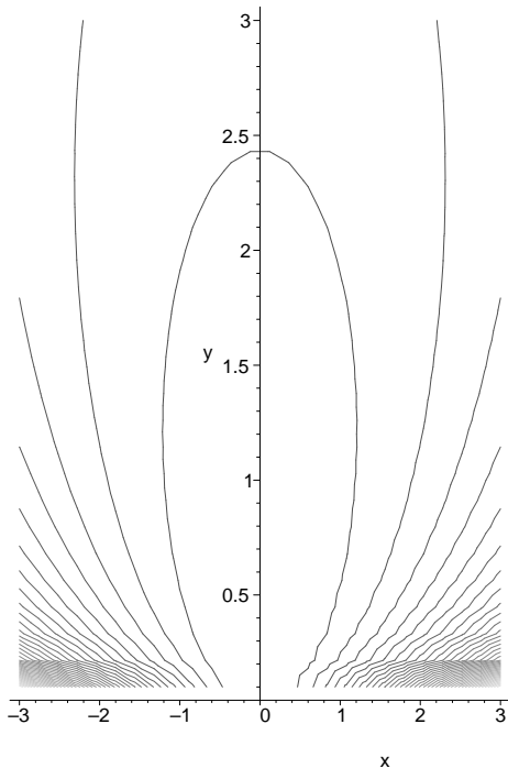
Figure 8: Contour plot of the potential generated by a brane wrapping the q_0 = 0, q = 0, q_0 = 1 cycle in a four dimensional factorizable torus with the same complex structure in the two 2-tori.
