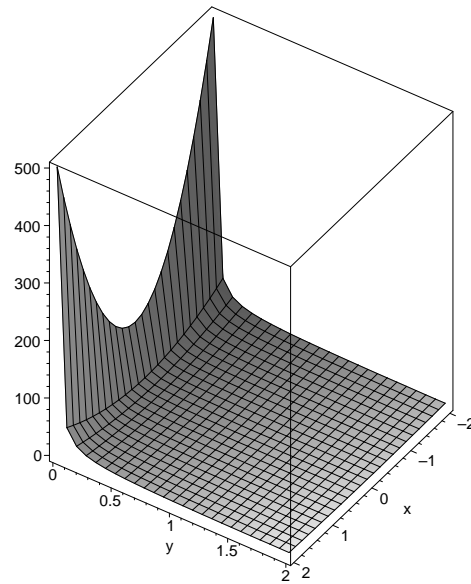
Figure 11: Three dimensional representation of the potential generated by a brane wrapping the q_0 = 1, q = 0, q_0 = 1 cycle in a four dimensional factorizable torus with the same complex structure in the two 2-tori.
