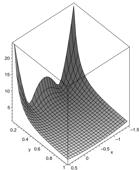
Figure 19: Three dimensional representation of the potential generated by a brane wrapping the q_0 = 0, Q = 0, P = 0, p^0 = 1 cycle in a six dimensional factorizable torus with the same complex structure in the three 2-tori.
