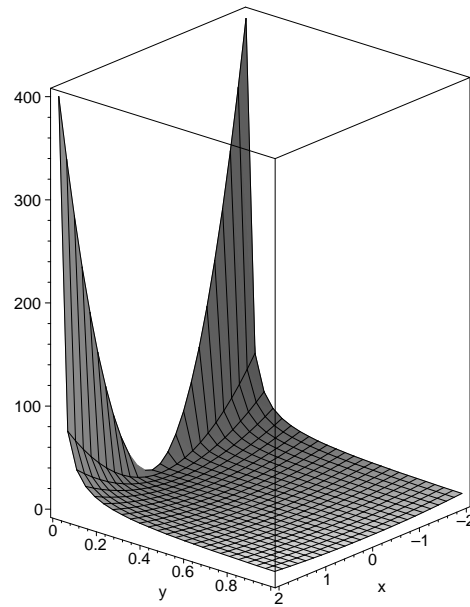
Figure 9: Three dimensional representation of the potential generated by a brane wrapping the q_0 = 0, q = 0, q_0 = 1 cycle in a four dimensional factorizable torus with the same complex structure in the two 2-tori.
