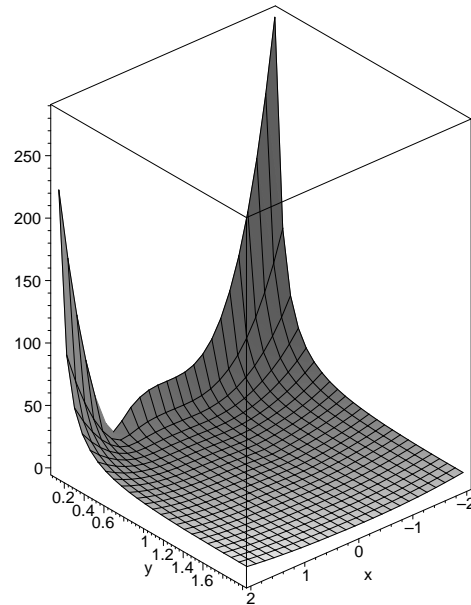
Figure 17: Three dimensional representation of the potential generated by a brane wrapping the q_0 = 1, q_1 = 0, p = 0, p^0 = 1 cycle in a six dimensional factorizable torus with the same complex structure in the three 2-tori.
