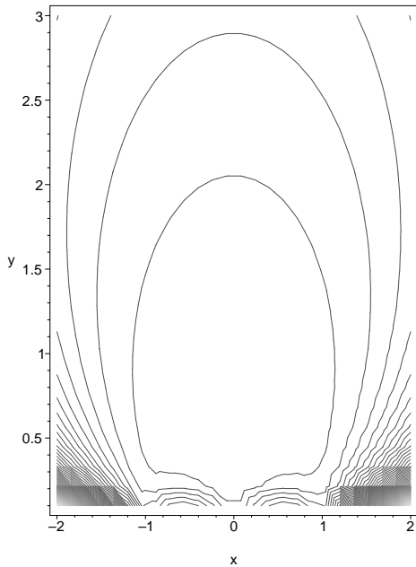
Figure 12: Contour plot of the potential generated by a brane wrapping the q_0 = 0 , q_1 = 1=3 , p = 0 , p^0 = 1 cycle in a six dimensional factorizable torus with the same complex structure in the three 2-tori.
