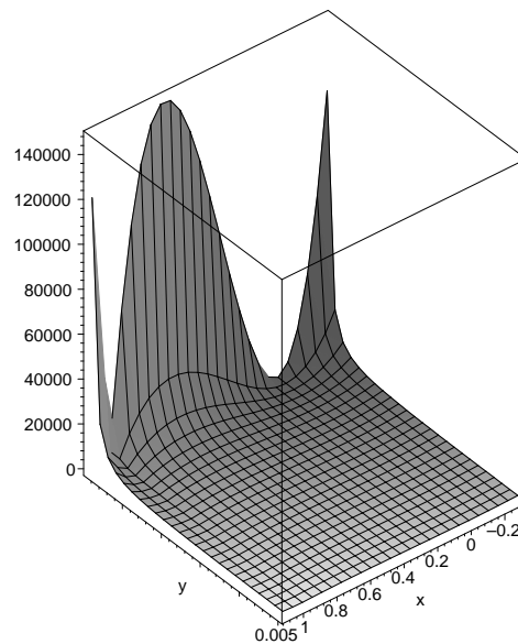
Figure 15: Three dimensional representation of the potential generated by a brane wrapping the q_0 = 0, q_1 = 0, p = 1=3, p^0 = 1 cycle in a six dimensional factorizable torus with the same complex structure in the three 2-tori.
