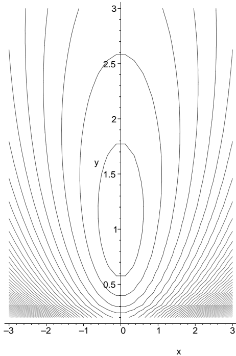
Figure 10: Contour plot of the potential generated by a brane wrapping the q_0 = 1, q = 0, q_0 = 1 cycle in a four dimensional factorizable torus with the same complex structure in the two 2-tori.
