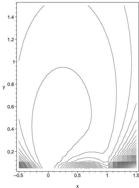
Figure 14: Contour plot of the potential generated by a brane wrapping the q_0 = 0, q_1 = 0, p = 1=3, p^0 = 1 cycle in a six dimensional factorizable torus with the same complex structure in the three 2-tori.
