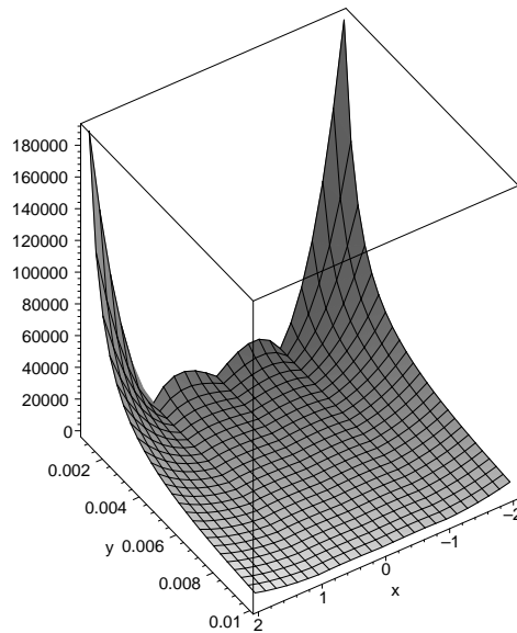
Figure 13: Three dimensional representation of the potential generated by a brane wrapping the q_0 = 0 , q_1 = 1=3 , p = 0 , p^0 = 1 cycle in a six dimensional factorizable torus with the same complex structure in the three 2-tori.
