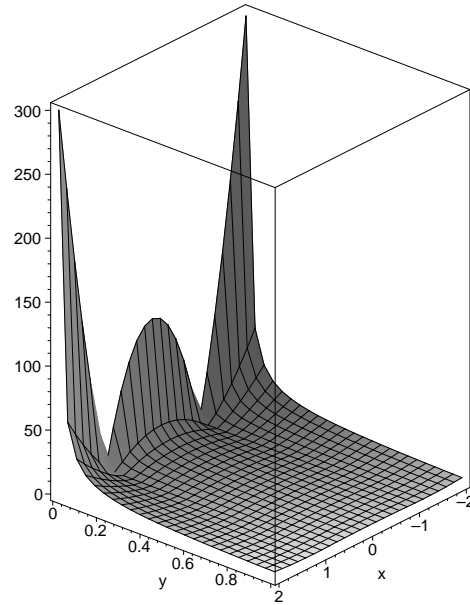
Figure 7: Three dimensional representation of the potential generated by a brane wrapping the q_0 = 1, q = 0, q_1 = 1 cycle in a four dimensional factorizable torus with the same complex structure in the two 2-tori.
