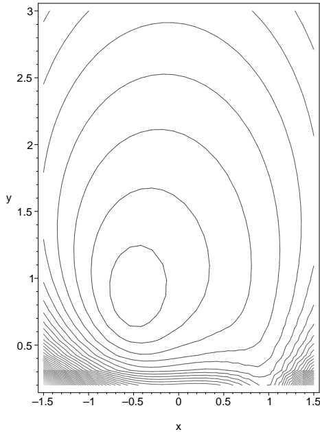
Figure 16: Contour plot of the potential generated by a brane wrapping the q_0 = 1, q_1 = 0, p = 0, p^0 = 1 cycle in a six dimensional factorizable torus with the same complex structure in the three 2-tori.
