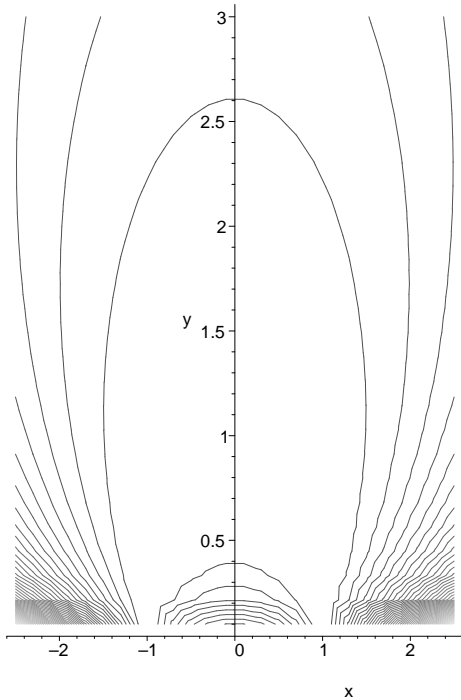
Figure 6: Contour plot of the potential generated by a brane wrapping the q_0 = 1, q = 0, q_1 = 1 cycle in a four dimensional factorizable torus with the same complex structure in the two 2-tori.
