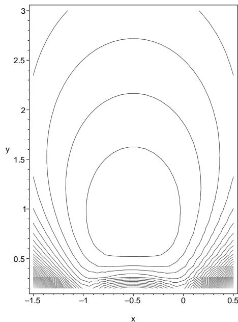
Figure 18: Contour plot of the potential generated by a brane wrapping the q_0 = 0, Q = 1, P = 1, p^0 = 0 cycle in a six dimensional factorizable torus with the same complex structure in the three 2-tori.
