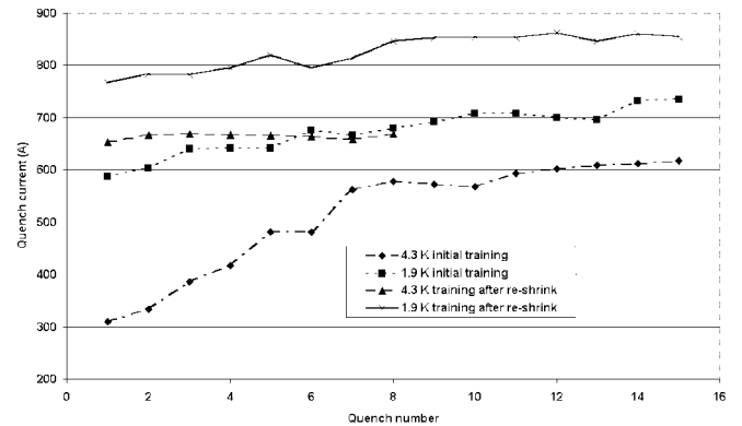
Fig. 6. MQTB training. After increasing the pre-stress the magnet reached the theoretical critical current at both 4.3 K and 1.9 K.
