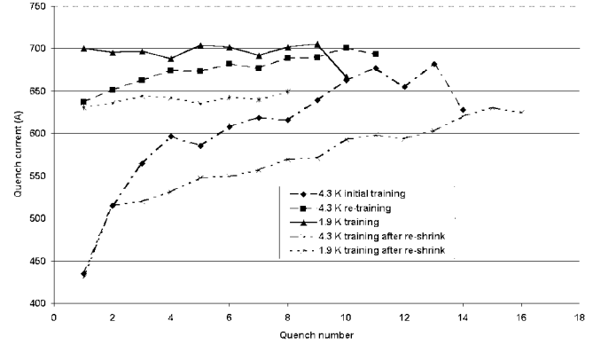
Fig. 5. MQTA training. No increase in the critical current is observed at 1.9 K, indicating a mechanical limitation to the magnets' performance.
