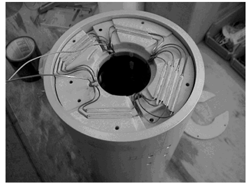
Fig. 3. MQTB electrical connections. Not only must the 4 coils be connected in series, but also the 6 layers in each coil.
