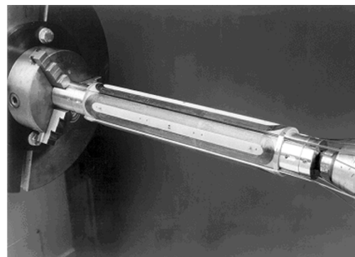
Fig.1. Assembly of MQTA coils. The coils are dowelled to a precisely machined mandrel. A glass fibre plate is mounted at the connection end to support the connections and the assembly glued together using epoxy resin.
