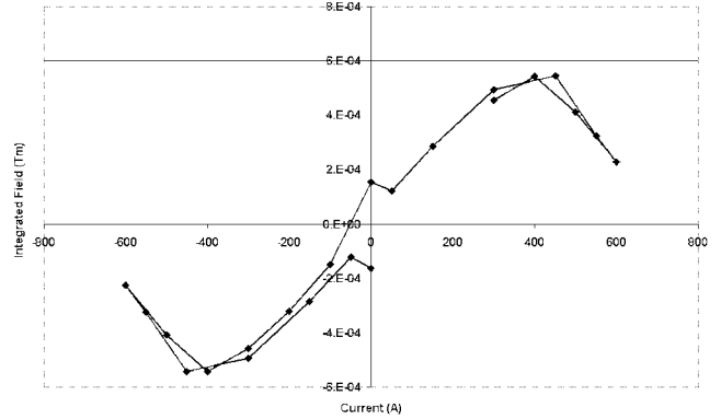
Fig. 10. Integrated B_6 harmonic of MQTB, at a reference radius of 17mm, measured passing through zero current from opposite directions.
