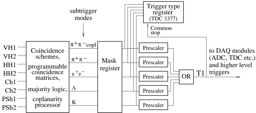
Fig. 3. Combination of different subtrigger modes in the 1st level trigger.
